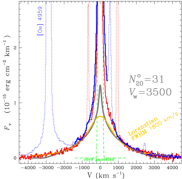
Fig. 8. Same notation as in Fig. 5 except for the TML model, which corresponds to a slower wind of V_w=3500\text{ km s}^{-1} with N_{20}^o=31 . For comparison, a Lorentzian profile of 1800\text{ km s}^{-1} FWHM is overlaid.
