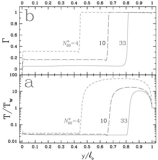
Fig. 3. Behavior in panel a of the temperature normalized to the value in the wind and in panel b of \Gamma (Eqn. 7), both as a function of the normalized thickness y/l_o . The three models shown vary only by their mixing layer nominal column: N_{20}^o = 4, 10 and 33 .
