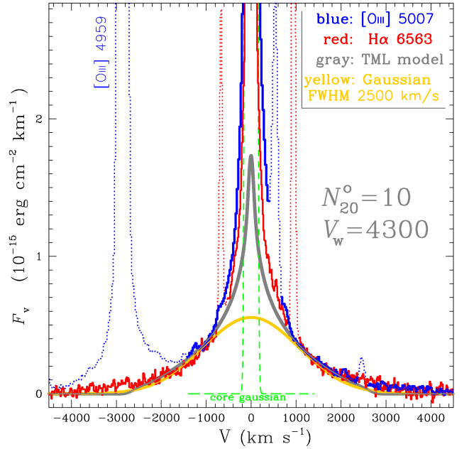
Fig. 5. Superposition of the emission line profiles of H\alpha (red line) and of [O\text{ III}]\lambda 5007 (blue line) as a function of Doppler velocity with respect to the centroid of both lines. The scale applies to H\alpha and the units are \text{erg cm}^{-2} \text{ km}^{-1} . The [O\text{ III}] profile has been scaled up so that its broad wings coincided as much as possible with those of H\alpha . Emission lines involving other energy levels have been partially blanketed with dotted line contours. Using a thick gray line, we overlaid the 3D profile from a TML model with N_{20}^o = 10 and V_w = 4300 \text{ km s}^{-1} . The yellow line shows how a broad Gaussian of 2500 \text{ km s}^{-1} FWHM would compare. The green colored dashed-line is a \text{FWHM} = 110 \text{ km s}^{-1} Gaussian fit of the narrow core component.
