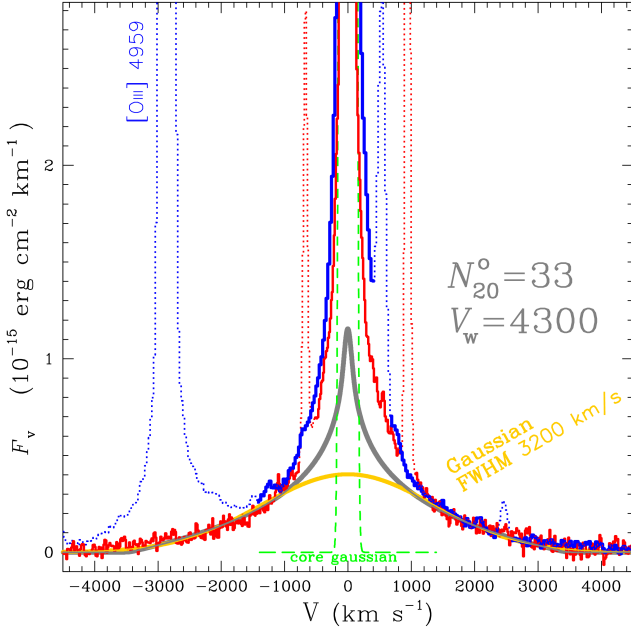
Fig. 6. Same notation as in Fig. 5 except for the TML model, which corresponds to N_{20}^o=33 . For comparison, a Gaussian of 3200 \text{ km s}^{-1} FWHM is overlaid.
