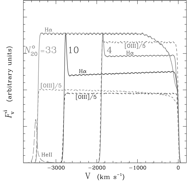
Fig. 4. Emission line flux from \text{H}\alpha (solid line) and [\text{O III}]\lambda 5007 (dashed line) as a function of radial velocity is plotted for each of the three models of Fig. 3. Note that the [\text{O III}] fluxes have been scaled down by a factor 5. The \text{He II } \lambda 4686 emission flux is shown in the case of the N_{20}^o = 33 model only.
