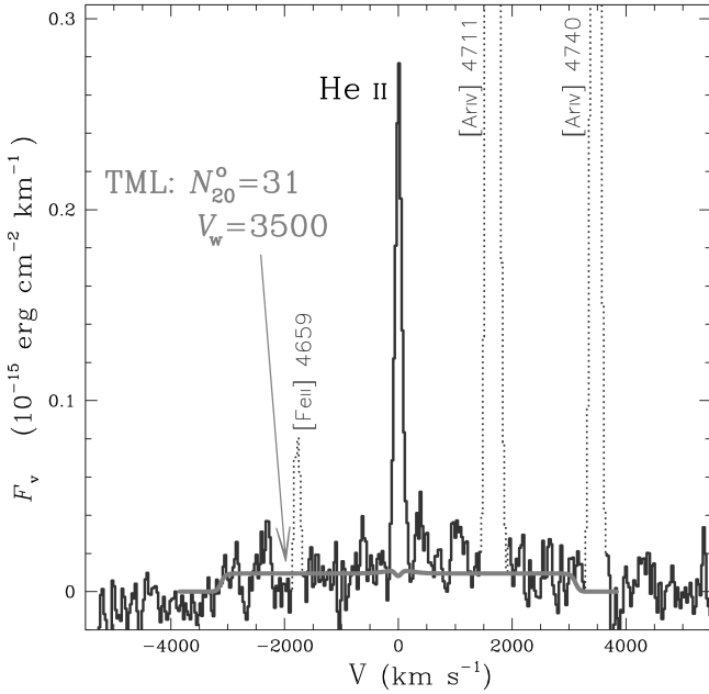
Fig. 9. Observed emission line profiles of He II \lambda 4686 (black line) as a function of Doppler velocity with respect to the centroid of both lines. Other line transitions near He II have been blanketed by dotting the corresponding line. We overlay a 3D profile from a TML model (gray line) with V_w = 3500 \text{ km s}^{-1} and N_{20}^o = 31 , but with its intensity multiplied by a factor 5.
