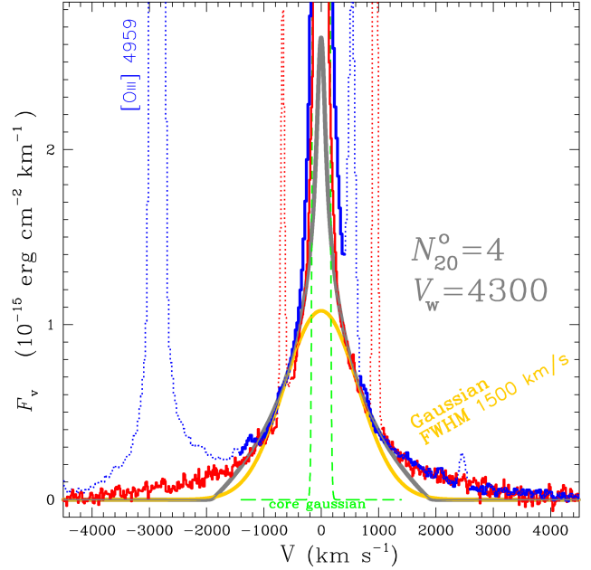
Fig. 7. Same notation as in Fig. 5 except for the TML model, which corresponds to N_{20}^o=4 . For comparison, a Gaussian of 1500 \text{ km s}^{-1} FWHM is overlaid.
