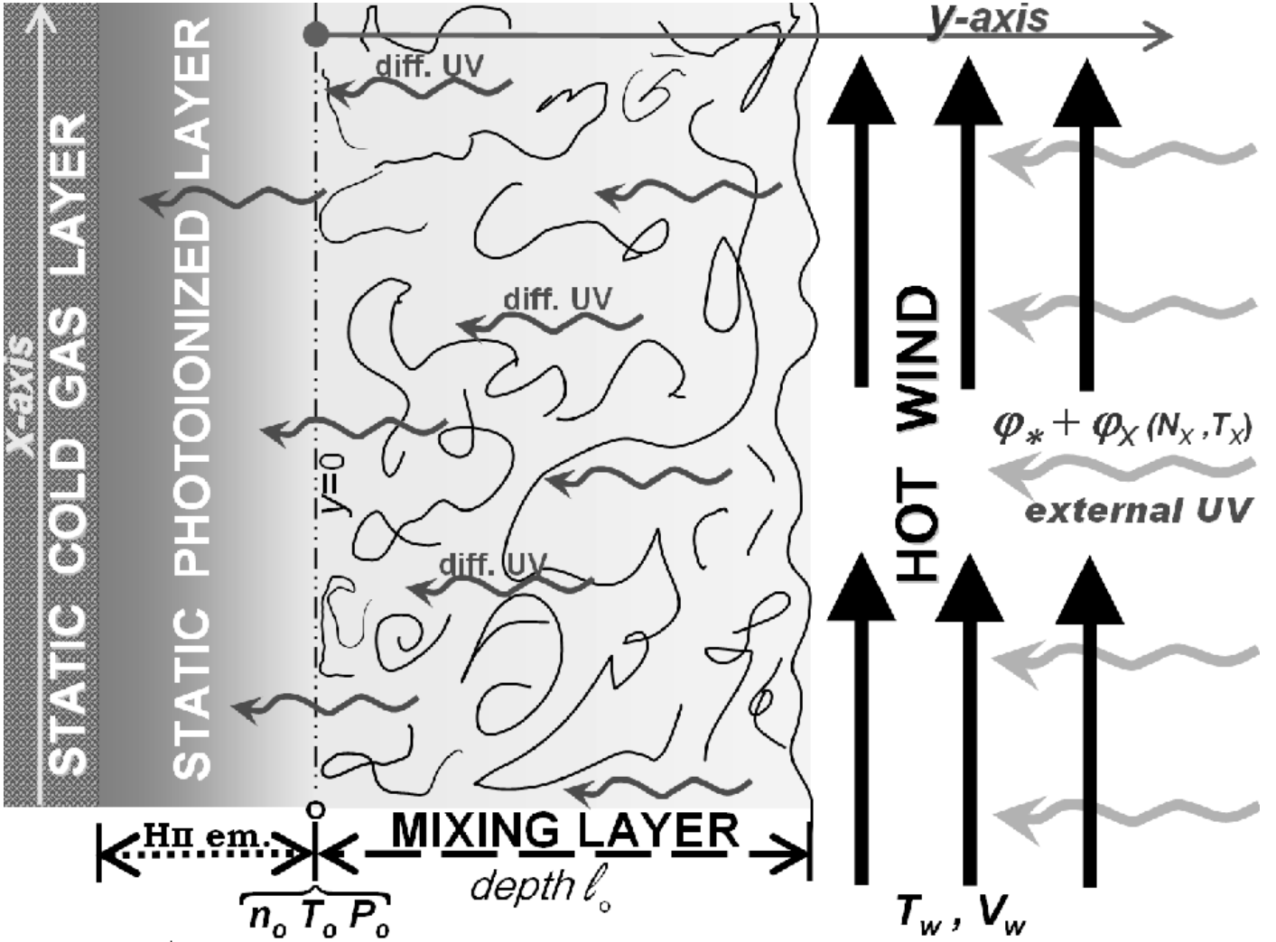
Fig. 2. Schematic diagram showing the cross-section along the y -axis of a plane-parallel mixing layer of thickness l_o . The mixing layer is formed by the interaction of a supersonic wind (velocity V_w and temperature T_w ) with a static layer of warm gas of H number density n_o and temperature T_o (at y = 0 ).
