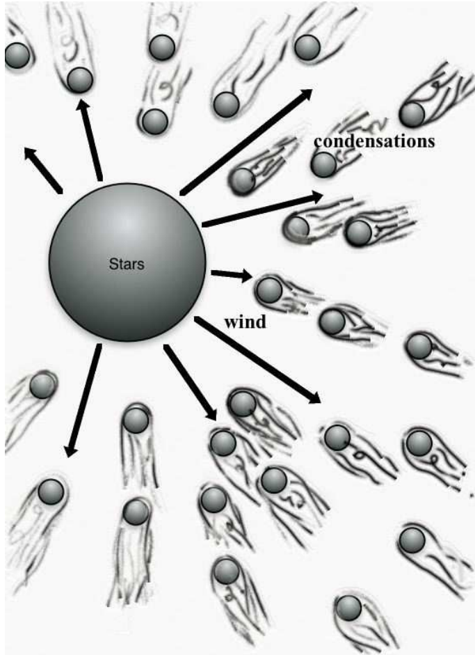
Fig. 1. The drawing describing the geometry of the super-cluster hot wind within which photoionized condensations are distributed.
