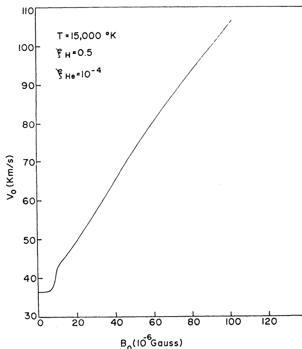
FIG. 3. The shock velocity that will produce a 50% ionization of hydrogen as a function of the pre-shock magnetic field. The post shock temperature is 15\,000 \text{ K} and the ionization of helium is approximately 10^{-4} .
