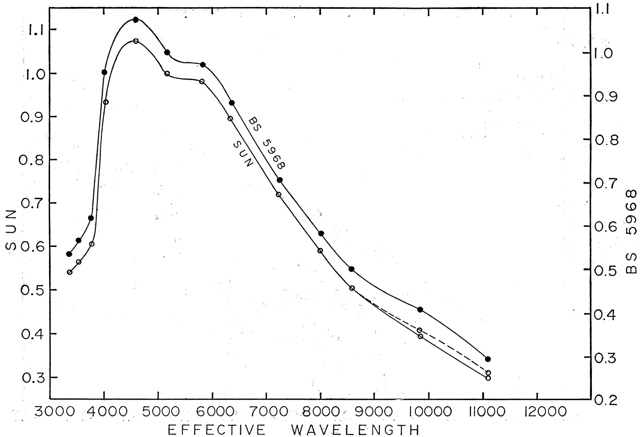
FIG. 3. F(\lambda)/(5180\text{\AA}) versus the effective wavelength (in angstroms) for the Sun (open circles) and for BS5968 (filled circles). That is, the ordinate is a linear flux density scale normalized at the 52 filter. The curves are derived using the energy calibration of Mitchell and Johnson, (1969, Table 2) and so are independent of the response curves of the phototubes. In the infrared the solid line for the Sun represents the photometry of Table 6A while the dotted line represents the revised values mentioned in the text.
