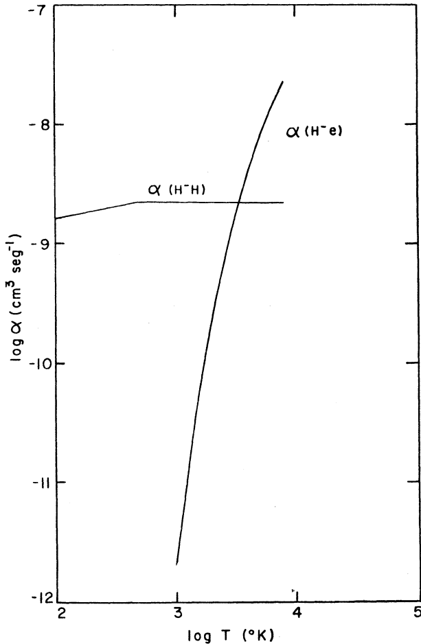
FIG. 2. Rate coefficients of the reactions \text{H}^- + e \rightarrow \text{H} + 2e and \text{H}^- + \text{H} \rightarrow \text{H}_2 + e as a function of temperature for 100^\circ\text{K} \leq T \leq 8000^\circ\text{K} .
