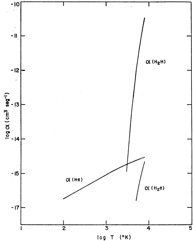
FIG. 1. Rate coefficients for the reactions H+e \rightarrow H^- + \gamma , H_2+H \rightarrow 3H and H_2+e \rightarrow H+H^- as a function of temperature for 100\text{K} \leq T \leq 8000\text{K} .
