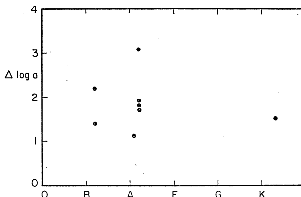
FIG. 4. Values of \Delta \log a vs type of brightest component for multiple stars.
