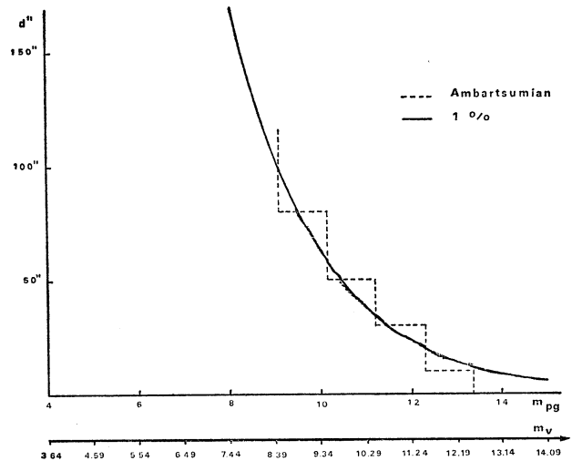
FIG. 1. Ambartsumian's filter (broken line) and 1% filter (solid line) for the direction l^I = 210^\circ , b^I = 5^\circ .
