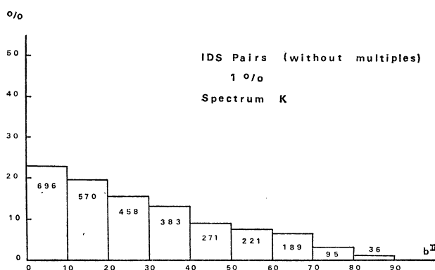
FIG. 14. Distribution in galactic latitude of pairs from the IDS of spectral type K, after removing multiples (1% filter).
