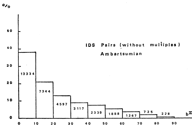
FIG. 5. Distribution in galactic latitude of pairs from the IDS after removing multiples (Ambartsumian's filter).
