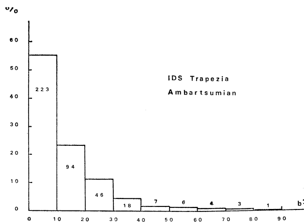
FIG. 3. Distribution in galactic latitude of trapezia from the IDS (Ambartsumian's filter). In this and all successive figures the number of systems in each bin is indicated.
