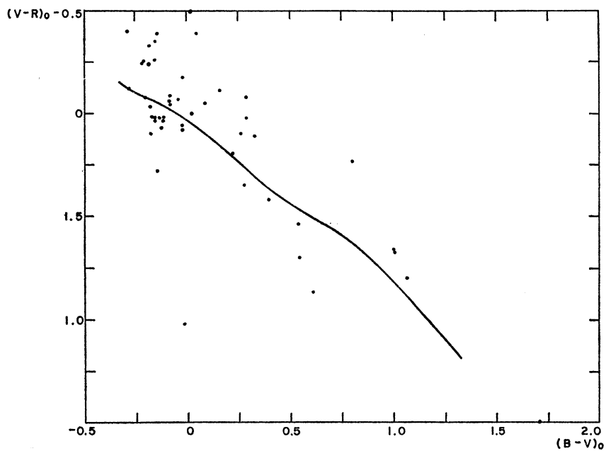
FIG. 4. Plot of (V - R)_0 versus (B - V)_0 .
