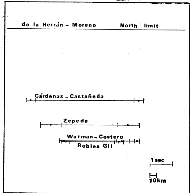
FIG. 2. Path of \gamma Ceti behind (6) Hebe, as seen from various locations.
