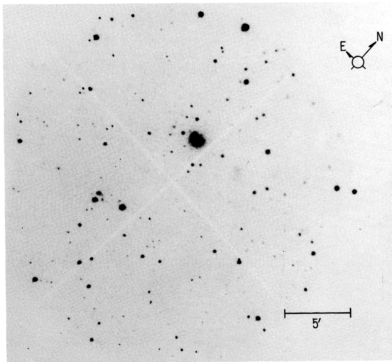
Fig. 3. [O III] spur in the neighborhood of the optical filaments presumably associated to the SNR CTB 13.
