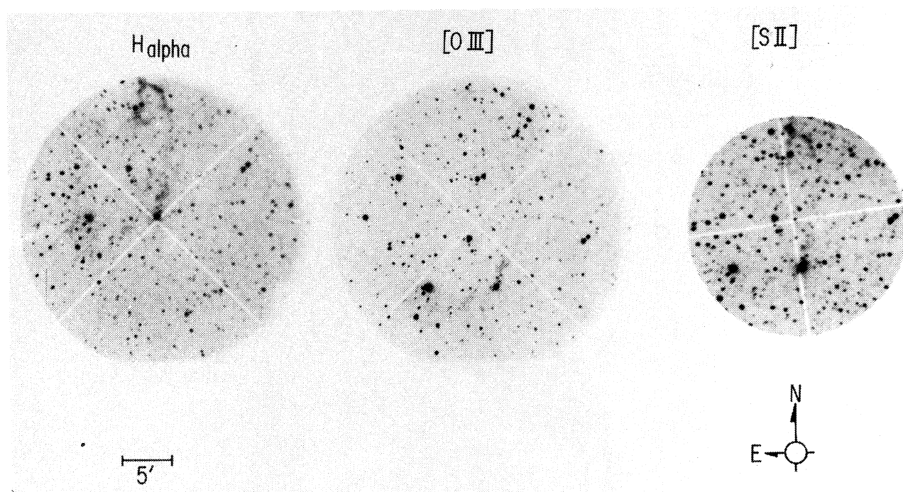
Fig. 1. H\alpha , [O III] and [S II] photographs of the SNR G126.2+1.6. The field for the [S II] photograph is smaller than the fields covered by the H\alpha and [O III] photographs due to the size of the [S II] filter.
