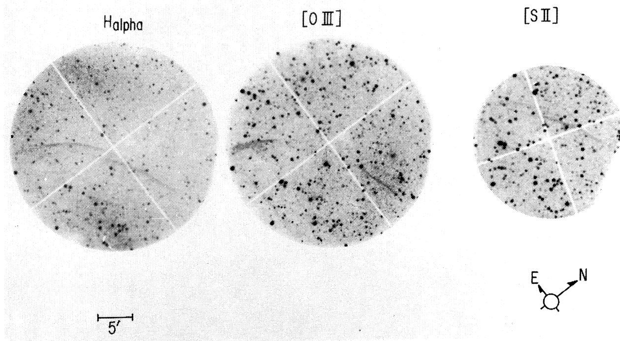
Fig. 2. The same as in Figure 1 but for the SNR G206.9+2.3.
