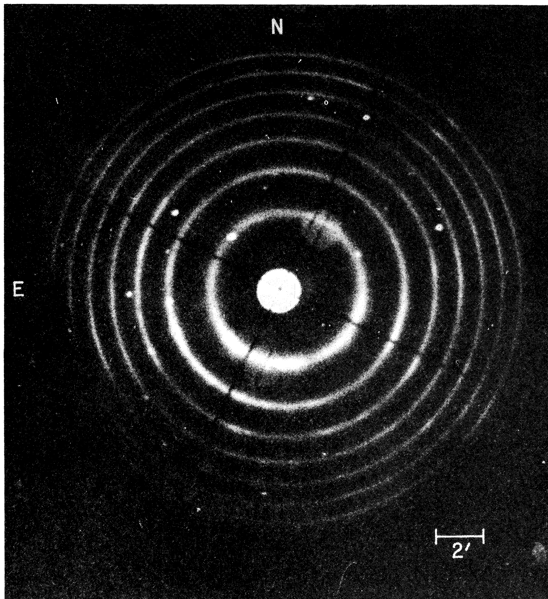
Fig. 1. Enlargement of an H\alpha interferogram (F 173) of the H II region S261 with an étalon giving an inter-order separation of 283 \text{ km s}^{-1} and using the 1 meter reflector at Tonantzintla Observatory.
