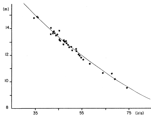
Fig. 1. Calibration curve for the first plate.
