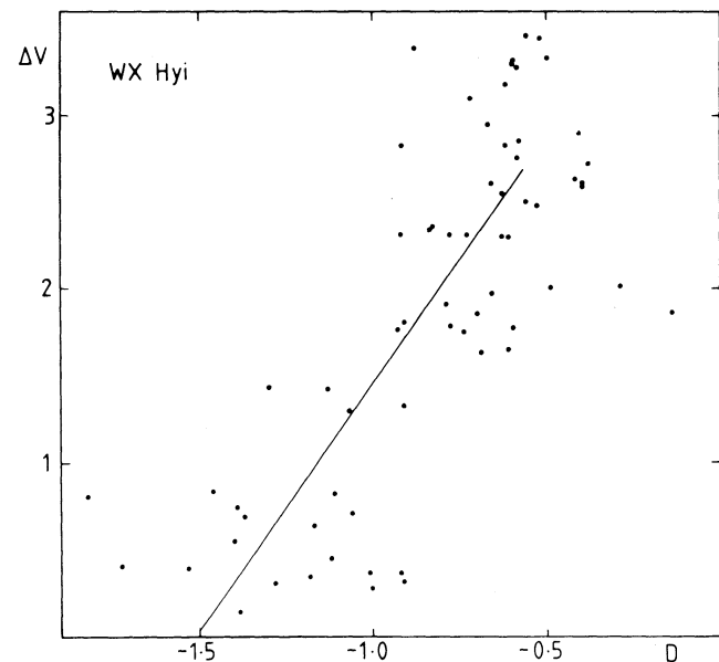
Fig. 9. Balmer discontinuity index versus change in visual magnitude for WX Hyi (see text).
