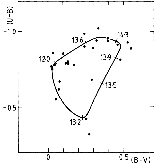
Fig. 2. Colour-colour diagram of AH Herculis. The V magnitude change during the outburst loop is shown.
