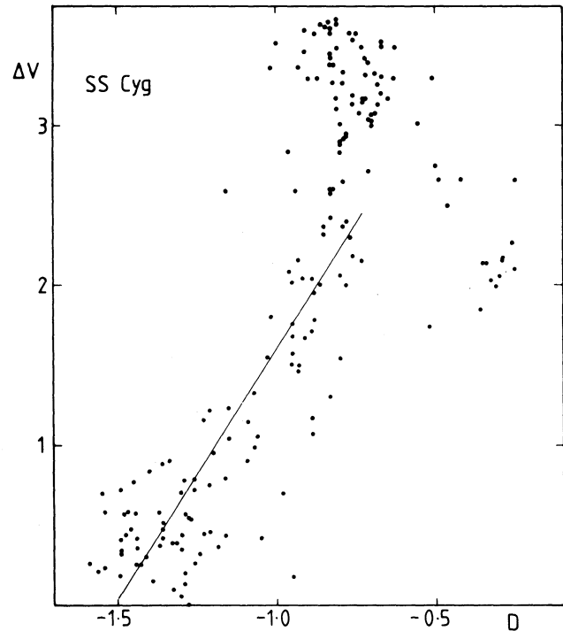
Fig. 8. Balmer discontinuity index versus change in visual magnitude for SS Cyg (see text).
