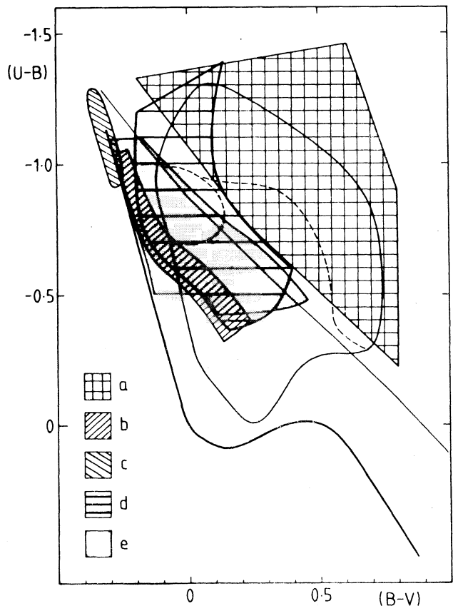
Fig. 4. Observational and theoretical (U-B, B-V) diagram. Models between the main-sequence and black body lines are optically thick. a) Tylenda 1981; b) Schwarzenberg-Czerny and Rozyzka 1977; c) Herter et al. 1979; d) Schwarzenberg-Czerny 1981; Mayo et al. 1980.
