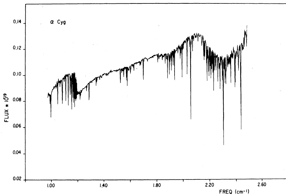
Fig. 4. The compressed spectrum of \alpha Cygni (see Figure 1).
