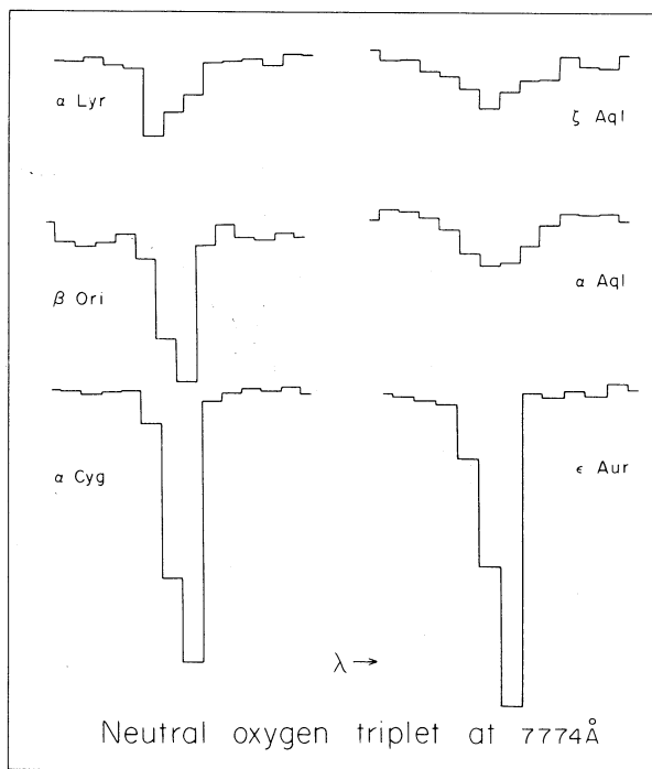
Fig. 8. The behavior of the neutral oxygen triplet line at 7774 \text{ \AA} in the six stars discussed in the text.
