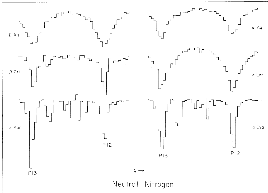
Fig. 9. The behavior of the neutral nitrogen lines in the near infrared (around \lambda 8700 \text{ \AA} ).
