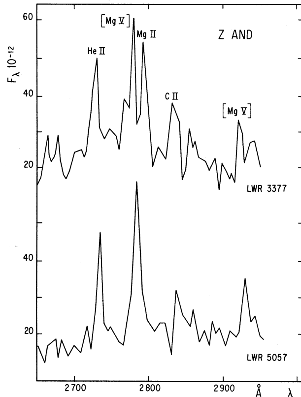
Fig. 2. Time variation of the spectral features of Z And in the 2650-2950 Å range.
