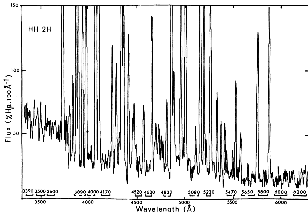
Fig. 6. The spectrum of H-H 2H obtained with the A.A.T. The spectrum is scaled to exhibit the continuum level (on this scale H \beta has an intensity of about 1500). Intervals chosen for continuum measurements are indicated. The emission lines (H, [S II], Mg I], Ca II, [Fe II], [O II], [O III], [N I], etc.) have been identified in previous studies (see Böhm et al. 1973). (From Dopita et al. 1982).
