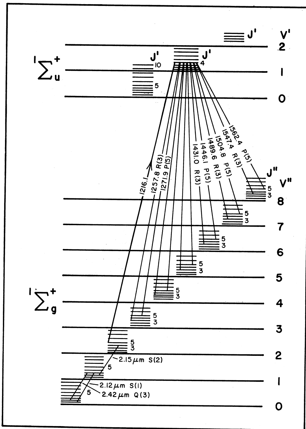
Fig. 11. A sketch of the energy states responsible for \text{H}_2 Lyman band fluorescence. The energy level separations are schematic only and do not represent a correct scaling. The pumping transition ( 1216.1 \text{ \AA} ) is about 0.38 \text{ \AA} longward of the central wavelength of \text{H Lyman } \alpha . The transitions to the v'' = 5, 4 states have wavelengths of \lambda 1387.4 \text{ P}(5) , \lambda 1372.5 \text{ R}(3) ; and \lambda 1329.1 \text{ P}(5) , \lambda 1314.6 \text{ R}(3) , respectively. However, the transition probabilities for these lines are low and the lines are not observed in \text{H-H } 43 or 47 . Whereas the UV lines represent electronic-vibrational-rotational transitions, the near IR lines seen in some \text{H-H} objects are vibrational-rotational transitions. Transitions detected by Elias (1980) are indicated between the first three vibrational states of the ground electronic state. Excitation of \text{H}_2 to the v'' = 1, 2 states evidently is caused by shock wave heating.
