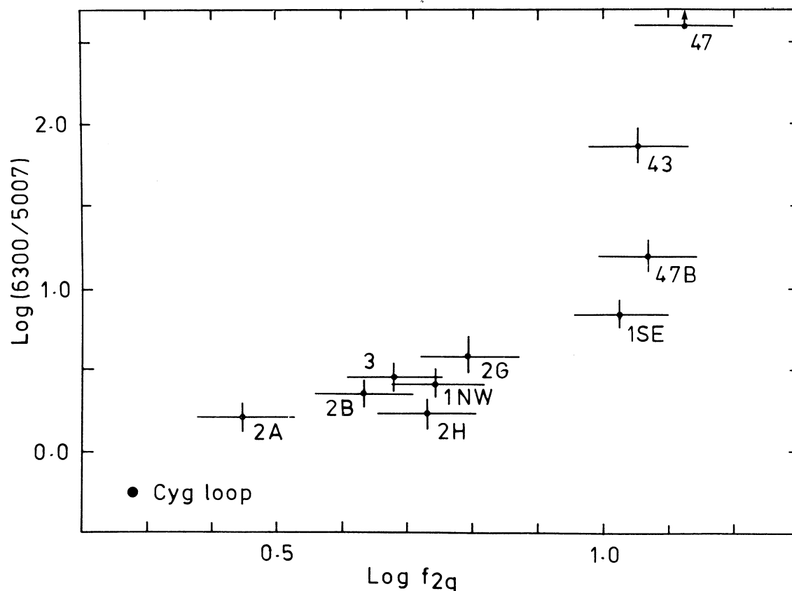
Fig. 9. The correlation of the 2q enhancement factor with the excitation state of H-H nebulae. The ordinate represents decreasing excitation with increasing values of the ratio [O\ I] \ 6300 / [O\ III] \ 5007 . (From Dopita et al. 1982).
