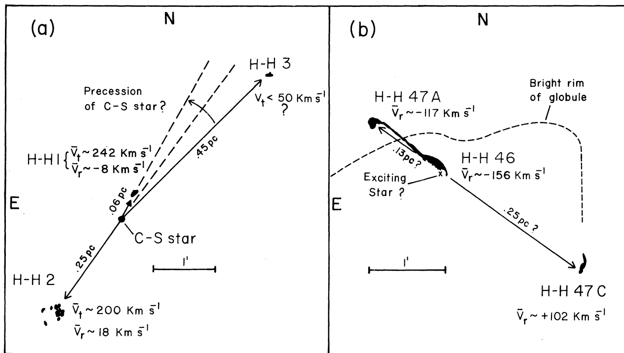
Fig. 13. The H-H 1-3 system (a) and the H-H 46-47 system (b), demonstrating the effect of quasi-periodic, alternate north and south polar ejections of H-H objects. A distance of 460 pc is assumed for H-H 1-3, and the globule associated with H-H 46-47 is assumed to be at a distance of 400 pc. Whereas the motions of H-H 1-3 are mostly in the plane of the sky, the radial velocities in H-H 46, 47A, and 47C suggest that the system has a significant inclination. The distance of H-H 47A and 47C from the exciting star are hence projected distances on the plane of the sky.
