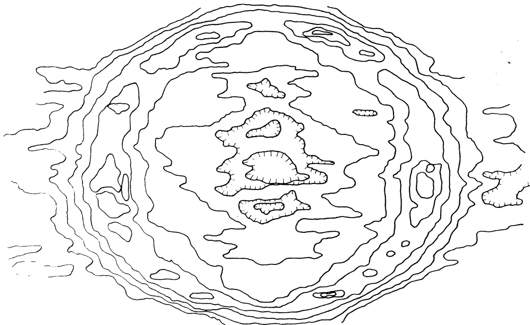
Fig. 5. Simulated neutral hydrogen shell with adjacent HI clouds, with different sizes and densities, randomly distributed. As in Fig. 2 the N_{\text{H}} levels are in arbitrary units.
