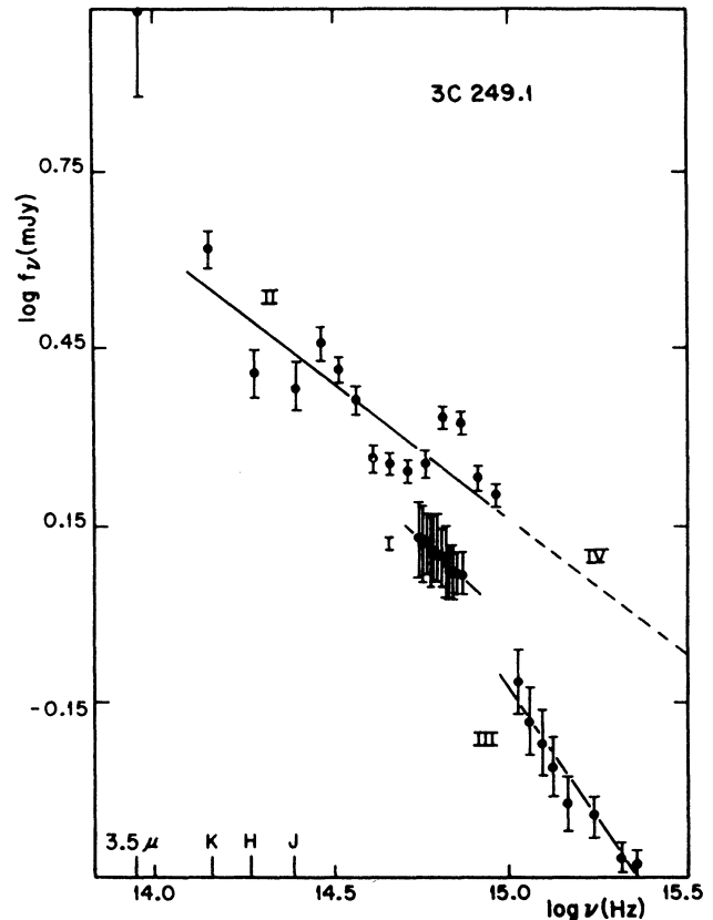
Fig. 4. Continuum energy distribution for 3C 249.1 I. This work; II. Neugebauer et al. (1979); III, IV. Dultzin-Hacyan et al. (1982).
