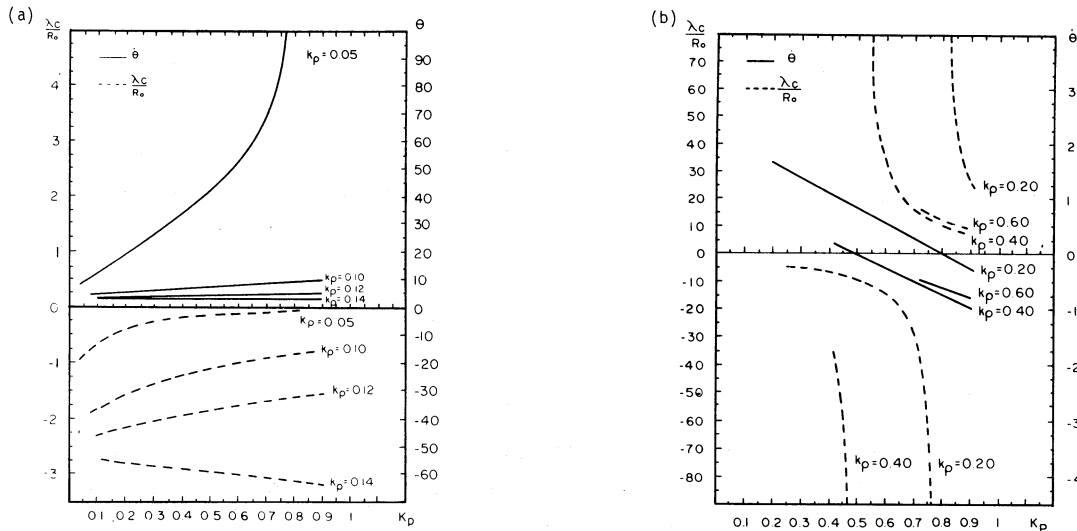
Fig. 3 - The rate of change of opening angle \dot{\theta} and the collimation length \lambda_c versus K_p = p_e/p_c for different values of K_\rho = \rho_0/\rho_c , with \theta = 4.9^\circ , M_z = 12 , M_{Az_c} = 16 and K_{v\phi} = 0 . In Fig. 3a we have K_\rho = 0.05, 0.10, 0.12 and 0.14 , and in Fig. 3b we have K_\rho = 0.2, 0.4 and 0.6 . Note the expanded scale of \dot{\theta} in Fig. 3b as compared with Fig. 3a.
