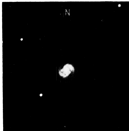
Fig. 2. The SBa galaxy, NGC 4314: a photograph taken on 103aE emulsion at the Cassegrain focus of the 2.1 meter reflector at San Pedro Mártir Observatory (Mexico). The tight nuclear spiral is clearly seen.
