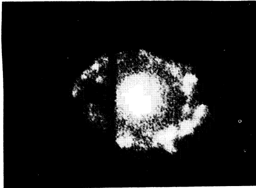
Fig. 3. The central spiral of NGC 4736 from an H\alpha interference filter ( 10 \text{ \AA} FWHM) photograph taken with a focal reducer attached to the 2.1 meter reflector at San Pedro Mártir Observatory (Mexico). Note the knotty nuclear spiral. The scale on the original plate is 49'' \text{ mm}^{-1}
