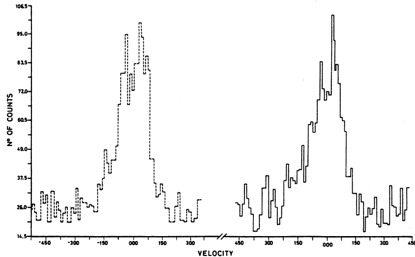
Fig. 2. Profiles of the H \alpha (solid line) and NII 6584 Å (dashed line) in a 3 arcsecond section of slit (width 0.5 arcsec) centred on the nucleus of NGC 6946.
