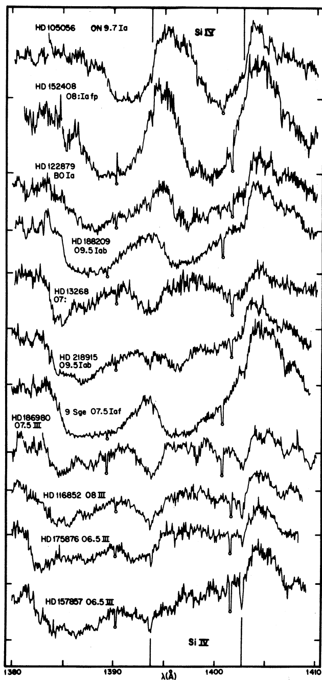
Fig. 2. Sequence of Si IV \lambda\lambda 1394\text{--}1403 profiles for the same stars in Figs. 1. The tick marks and the narrow vertical bars have the same meaning as in Fig. 1a.
