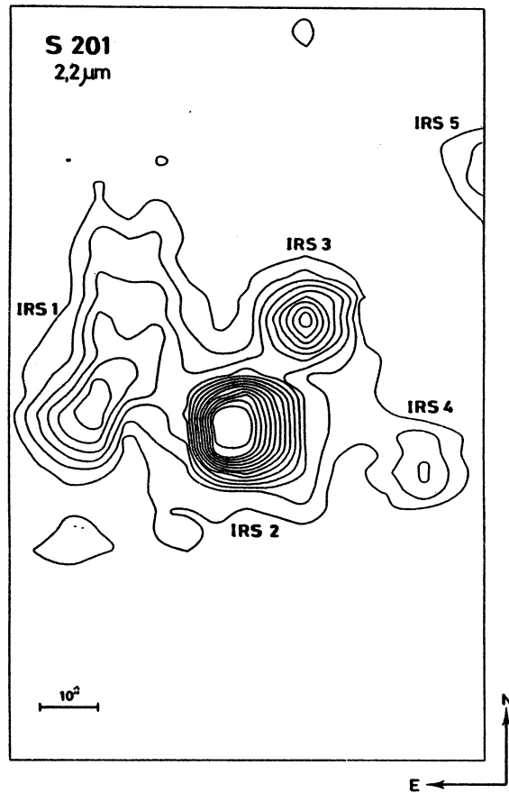
Fig. 4. 2.2 \mu m map of S201 showing the different sources discussed in the text.
