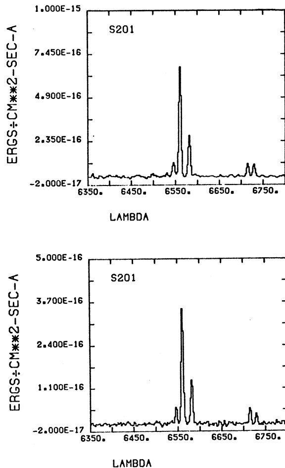
Fig. 3. Spectra of the bright optical north lobe (upper) and of the southern lobe (lower) of S201 in the zone of H \alpha . Note the difference in the relative ratio of the [SII] lines of the lobes.
