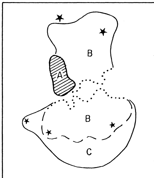
Fig. 2. Freehand sketch of the different subregions in S201, A, B and C, named in order of decreasing velocities.
