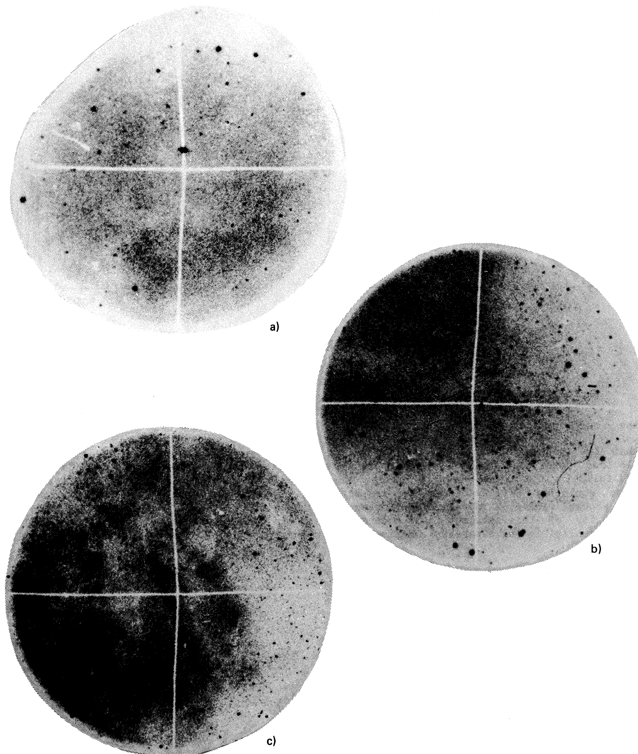
Fig. 1. H \alpha photographs of the nebulae: a) SG 196; b) Of #23; c) SG 154. In all cases the north is at top, east at right. The angular diameters of the pictures are for a) and b) \phi = 12' and for c) \phi = 30' .
