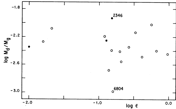
Fig. 6. Dust to gas ratio versus filling factor for the PN in Figure 5.
