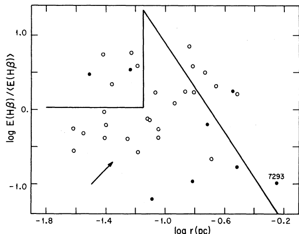
Fig. 7. \log E(\text{H}\beta) versus \log r diagram for the scale-independent sample. \langle E(\text{H}\beta) \rangle = 3.50 \times 10^{34} \text{ erg s}^{-1} . The horizontal line and the diagonal line correspond to the optically thick and optically thin distance scales respectively by Cudworth (1974). His optically thin scale crosses our optically thick scale at r = 0.20 \text{ pc} . The arrow indicates the displacement of any given point if its distance is increased by a factor of 1.4.
