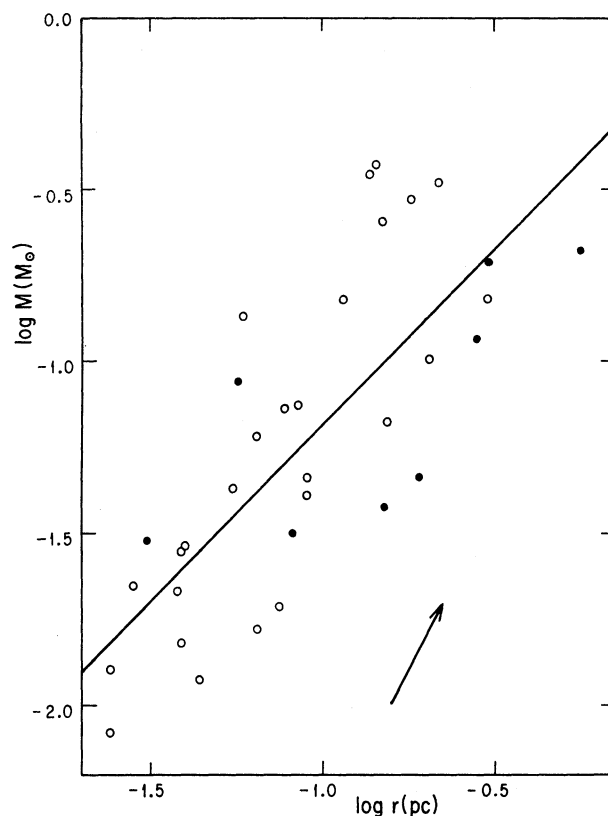
Fig. 4. Mass versus radius diagram for PN with scale-independent distances. Filled circles Type I PN, open circles the rest. The straight line is the least squares fitting to the data given by \log M(\epsilon) = (-0.16 \pm 0.17) + (1.02 \pm 0.15) \log r ; with a correlation coefficient of 0.77. The arrow indicates the change in mass if an object is 1.4 times farther away than assumed.
