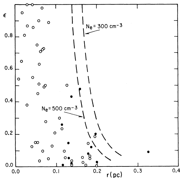
Fig. 2. Same as Figure 1 but for PN in Daub's (1982) sample adopting the Daub distance scale. The area to the right of the broken lines corresponds to optically thin PN with N_e(\text{FL}) smaller than 500 and 300 \text{ cm}^{-3} respectively.
