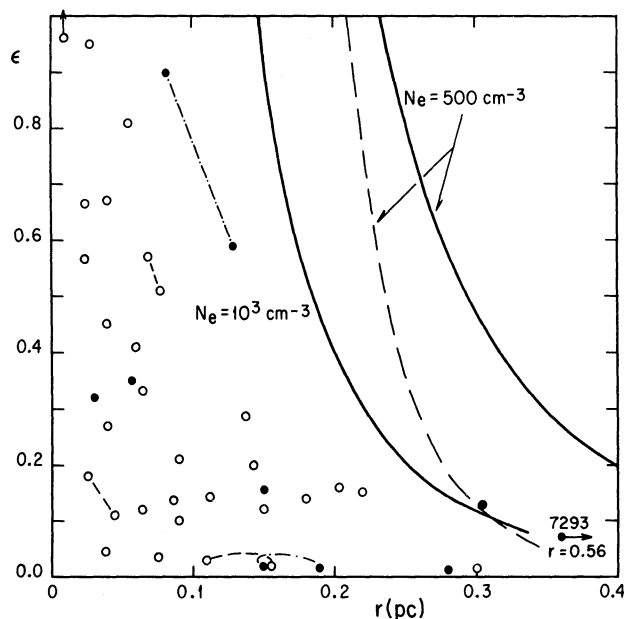
Fig. 1. Filling factor versus radius diagram for PN with scale-independent distances. Filled circles denote Type I PN, open circles the rest. Those circles joined by broken lines denote the same object with two different distance estimates as given in Table 1. The areas to the right of the solid lines correspond to optically thick PN with N_e(\text{FL}) smaller than 10^3 and 500 \text{ cm}^{-3} respectively, while the area to the right of the broken line corresponds to optically thin PN with N_e(\text{FL}) smaller than 500 \text{ cm}^{-3} (see text).
