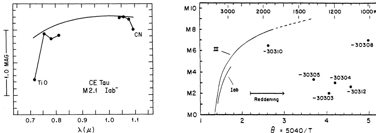
Fig. 2 (left). Eight-color photometry of the M supergiant 119 CE Tau. Absolute flux per unit wavelength interval, on a magnitude scale, is plotted against wavelength in microns. A blackbody curve for 2905 K has been fitted to the spectrum, with allowance for CN absorption at filter 2. Filters 1 and 8 are depressed by TiO and CN, respectively, leading to the classification M2.1 Iab-.
