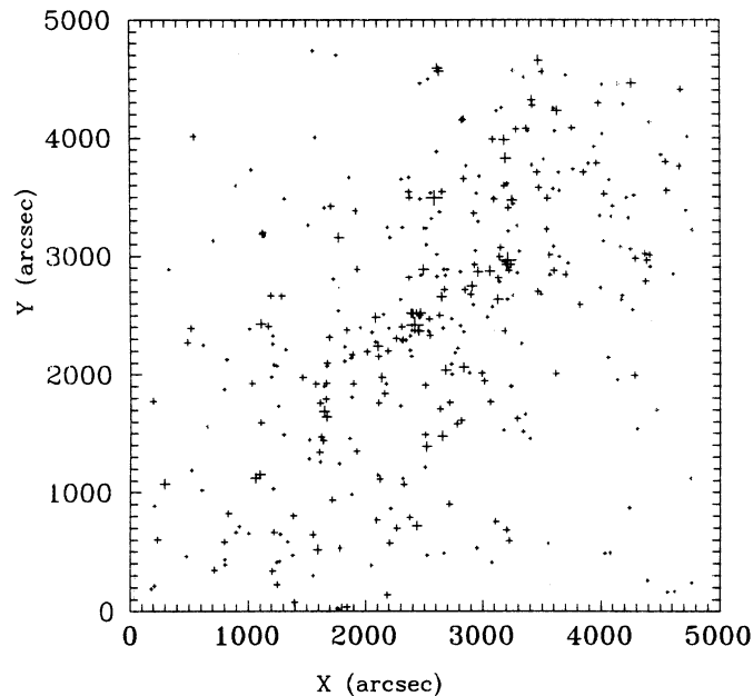
Fig. 1. Distribution of the galaxies of the catalogue. The cross dimensions are nearly proportional to galaxy luminosities. The brightest cluster galaxy is at the center of the figure (N top, E left).
