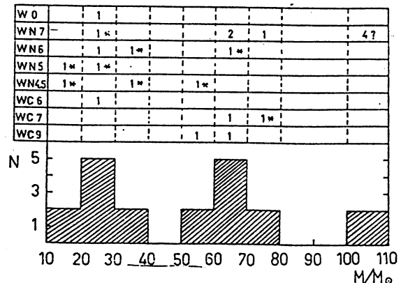
Figure 2. Distribution of initial masses for WR-type stars. The frequency of subtypes is indicated. The asterisk means binarity.
