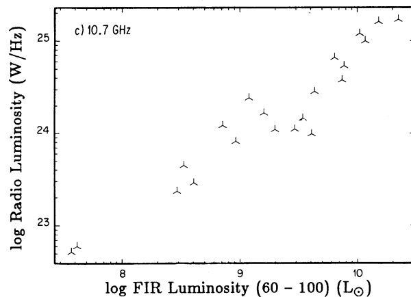
2. Radio luminosity versus IRAS far-infrared luminosity for the bright barred galaxies studied here. Note the tight relation between the two bands at every radio wavelength, a) 20 cm fluxes from Condon 1987; b) 6.3 cm fluxes, this work; c) 2.8 cm fluxes, this work.
