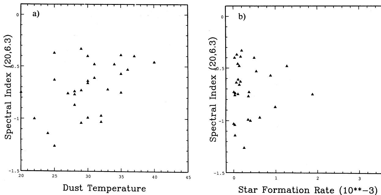
Fig. 4. a ) Spectral index \alpha_{20}^{6.3} versus dust temperature computed from IRAS 60 \mu m and 100 \mu m fluxes. Note that galaxies with T_d \geq 30^\circ\text{K} have \alpha_{20}^{6.3} > -0.75 except for NGC 4236, NGC 4535 and NGC 4654 and are of late Hubble type. b ) Spectral index \alpha_{20}^{6.3} versus star formation rate as listed in Table 3 and calculated using the FIR luminosity according to Scoville & Young (1983).
