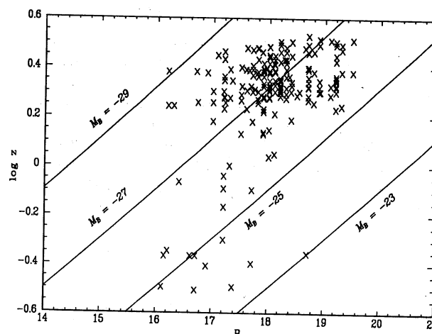
Fig. 4. Hubble diagram for Calán-Tololo quasars. 90% of the objects have M_B in the range -25 to -29 . Lines of absolute magnitudes were computed for H_0 = 60 \text{ km s}^{-1} \text{ Mpc}^{-1} , q_0 = 0.5 and \alpha = -0.5 .
