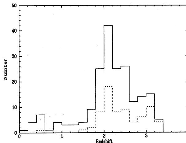
Fig. 2. Histogram of the redshift distribution of Calán-Tololo quasars. Solid line represents the total sample (200 objects); dashed line corresponds to the faint end of the sample ( B > 18.25 ) involving 70 objects. A total of 118 quasars (59%) have a redshift z such that 1.8 \leq z < 2.6 ; 173 quasars (86.5%) have z such that 1.6 \leq z < 3.4 .
