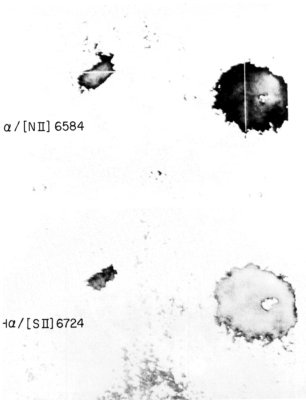
Fig. 2. (a) H\alpha/[N II] line ratio image. (b) H\alpha/[S II] line ratio image.
