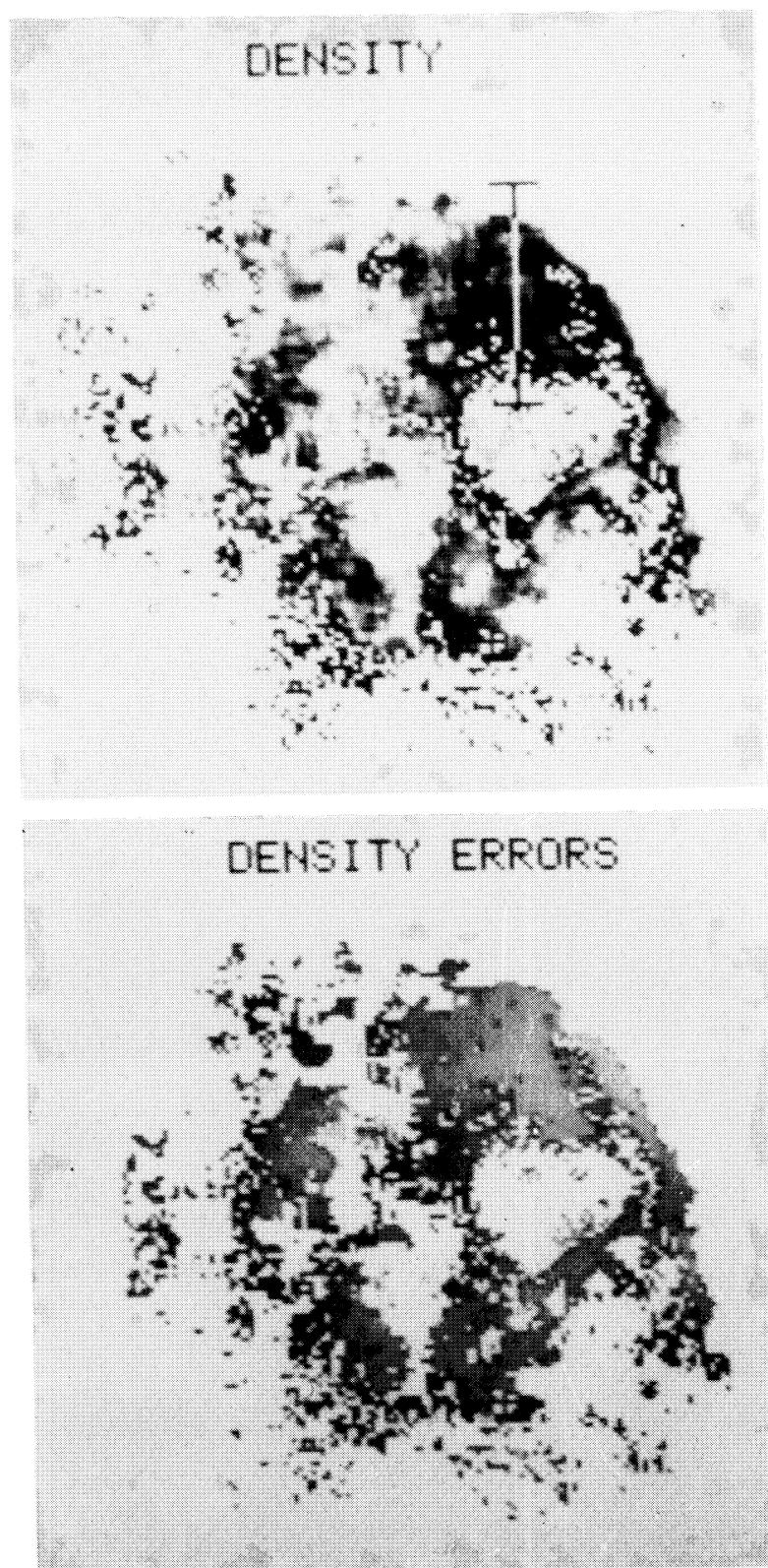
g. 5. (a) Density map of the western H II region. The density scale is shown to the right. (b) Error map for the density.
