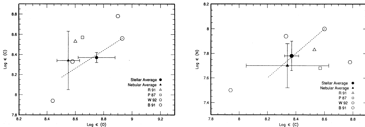
Figure 1 - (left) Comparative diagram of C/O ratios for Orion. The stellar average from B stars and the nebular average are shown with their respective error bars. The other symbols represent individual nebular ratios obtained in the literature (see table 2). The solar value is indicated with a solar C/O ratio for decreasing abundances, indicated by the dashed line.
