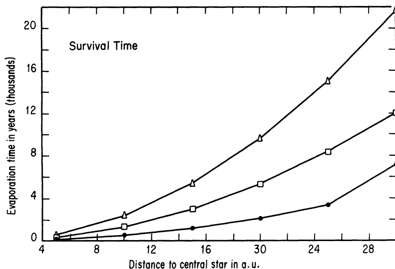
Fig. 2. Survival time.
