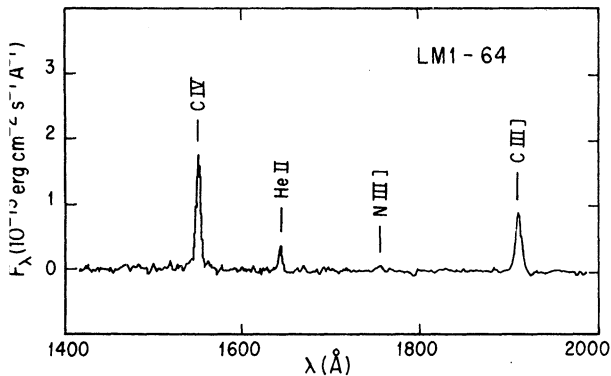
Fig. 3. Ultraviolet spectrum of LM1-64 resulting from the low dispersion exposures SWP 39573 (180 min) and WP 39576 (115 min).
