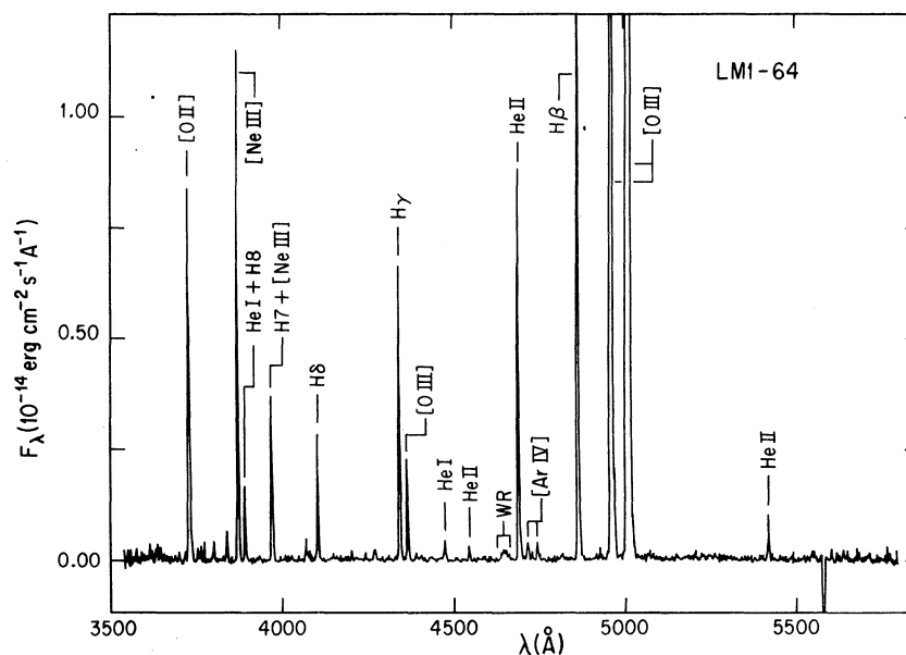
Fig. 2. Optical spectrum of LM1-64. The most important lines are indicated.
