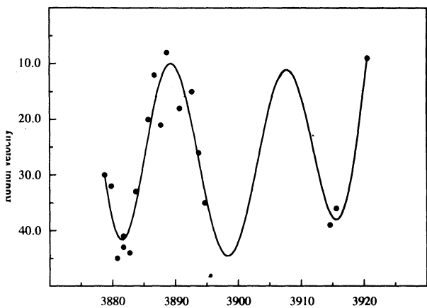
Fig. 3. Observations versus predictions (continuous line) for the spectroscopic data of Méndez & Niemela (1981). The prediction has been done using the frequencies determined from the photometric data.
