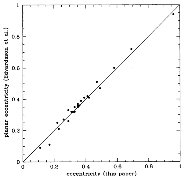
Fig. 4. Comparison of galactic orbital eccentricities obtained with two different mass models.
