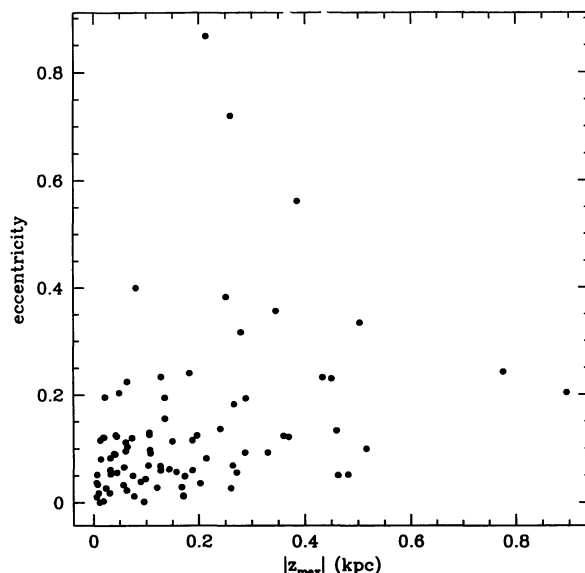
Fig. 10. Galactic orbital eccentricity versus |z_{\max}| for 93 nearby UV Ceti stars.
