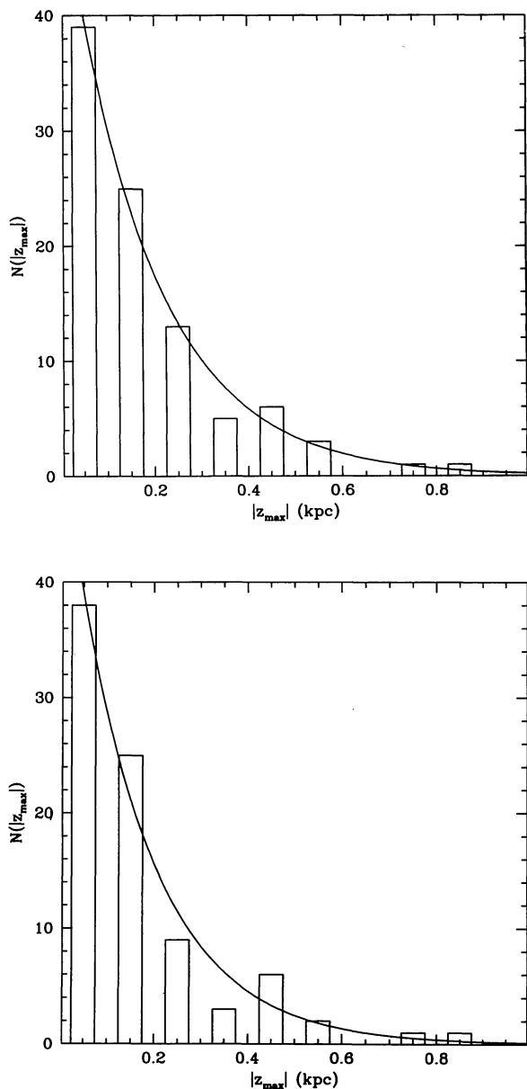
Fig. 9a). Histogram of |z_{\max}| for 93 nearby UV Ceti stars. The solid line is an exponential fit. b). Histogram of |z_{\max}| for 85 stars with e < 0.3 . The solid line is again an exponential fit.
