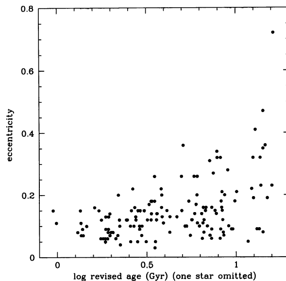
Fig. 7. Galactic orbital eccentricities versus ages for 143 disk stars having reliable ages according to Ng & Bertelli (1998).
