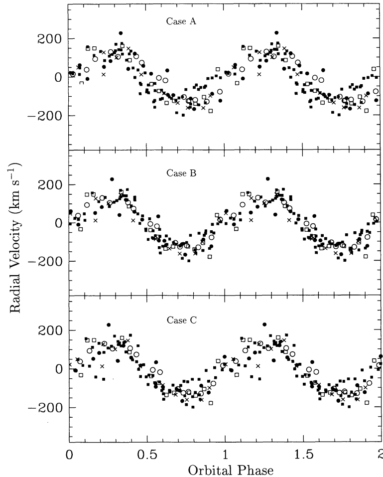
Fig. 2. Radial velocity curve of KT Per as a function of orbital phase for three different orbital periods, discussed in the text. Solid and open dots correspond to the H \beta data obtained by Ratering, Bruch, & Diaz (1993) on 1989, October 10 and 11, respectively. Crosses correspond to H \alpha observations by the same authors on 1989, October 12. Solid squares are H \alpha observations by Thorstensen & Ringwald (1997) obtained during several nights on 1989, November. Open squares correspond to our H \beta observations obtained on 1991, November 10.
