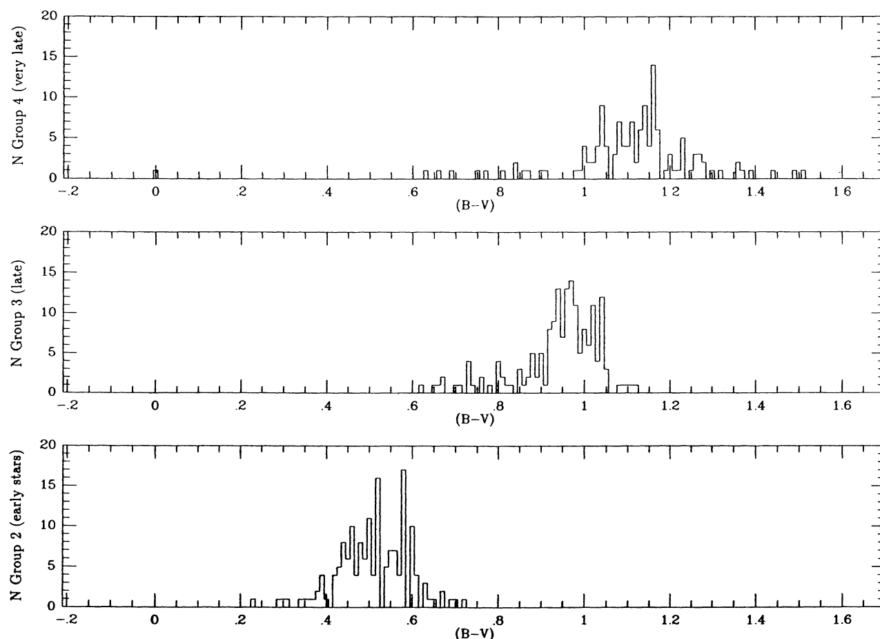
Fig. 6. Distribution of B - V after separating the different groups on the basis of line strength criteria.
