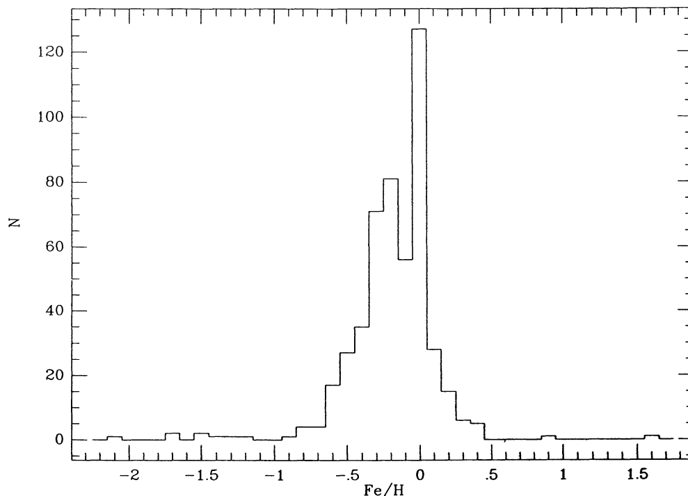
Fig. 3. Histogram of metallicities of all used stars in the Jones list.
