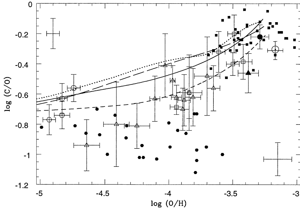
Fig. 5. \log(C/O) - \log(O/H) relation for r = r_{\odot} . The predictions of selected models (those that reproduce this relation) are presented as follows: dotted line : C-model, long-dashed line : MMBC2-model, continuous line : MRV1-model, short-dash line : MHG1-model. Observational data for the solar vicinity ( filled symbols ) are as follows: circle : Orion from Peimbert (1999); hexagons : field halo dwarfs from Tomkin et al. (1992); squares : dwarf stars from Gustafsson et al. (1999), as in Fig2; triangle : average B-star computed from the Gummersbach et al. (1998) data (as in Fig. 2); \odot : solar value from Grevesse & Sauval (1998). Error bars at the upper-left and the lower-right are typical errors from data by Gustafsson et al. (1999) and Tomkin et al. (1992), respectively. \log(O/H) for halo dwarfs is the average of [O/H] values from Tomkin et al. (1992). Observational data for external galaxies ( open symbols ) are as follows: circles : I Zw 18NW and I Zw 18SE, values adopted from Figure 4 of Garnett et al. (1999); hexagons : I Zw 18NW and I Zw 18SE, abundance ratios taken from Table 5 of Izotov & Thuan (1999); abundance data for spiral galaxies ( squares ) and dwarf irregular galaxies and Magellanic Clouds ( triangles ) are obtained from Garnett et al. (1999). Plotted C/O values for spiral galaxies are the average of the abundance ratios for two different reddening laws.
