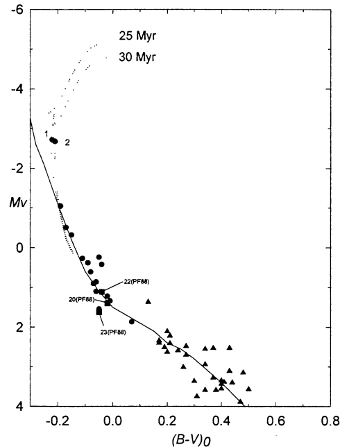
Fig. 6. The H-R diagram of likely and probable members of Trumpler 21. Solid line represents the Schmidt-Kaler's (1982) ZAMS fitted using a distance modulus of 10.7. Dotted lines are the isochrones from Schaller et al. (1992), their corresponding ages being indicated.
