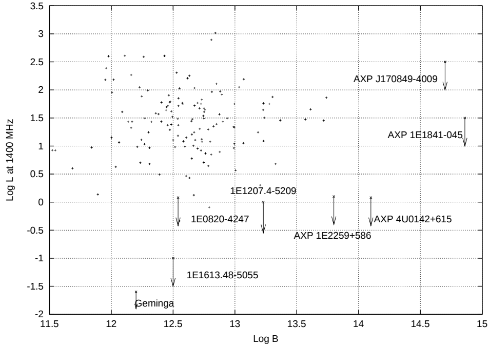
Fig. 6. The radio luminosity versus magnetic field strengths ( \text{Log } L_{1400} - \text{log } B ) for young PSRs ( \tau < 3 \cdot 10^5 yr) and different types of single point X-ray sources.
