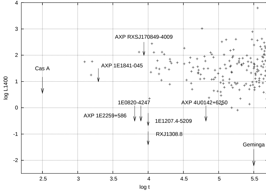
Fig. 5. The radio luminosity versus characteristic ages ( \log L_{1400} - \log \tau ) for young PSRs and for different types of single point X-ray sources.
