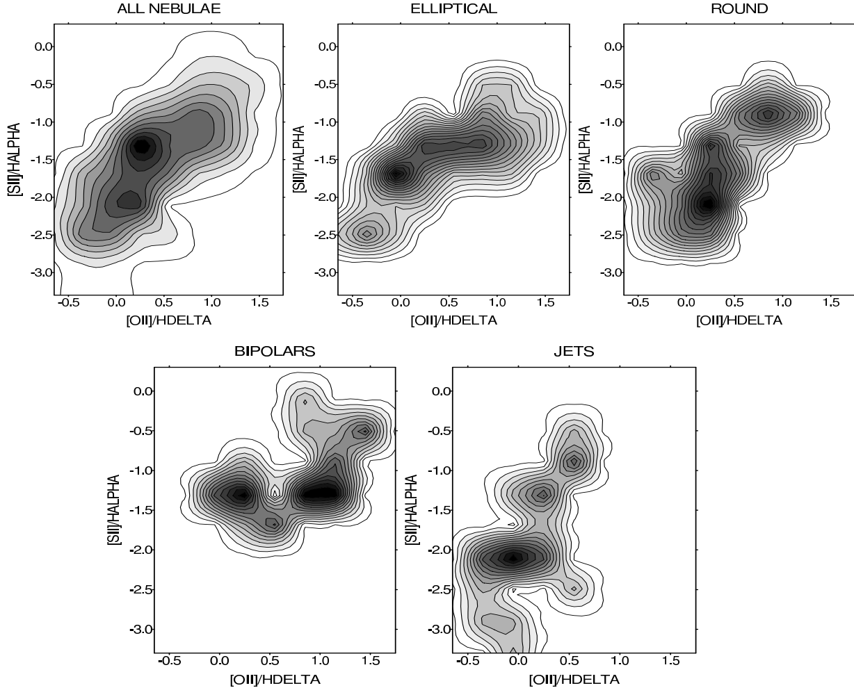
Fig. 2. As in Fig. 1, but for the [S II]/H\alpha – [O II]/H\delta plane.
