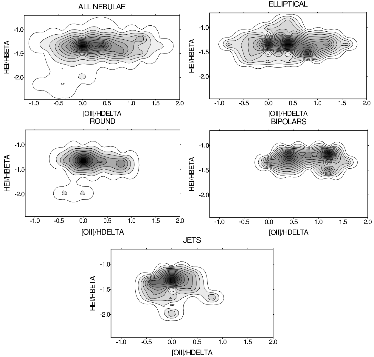
Fig. 3. As for Fig. 1, but for the \text{He I}/\text{H}\beta – [\text{O II}]/\text{H}\delta plane.
