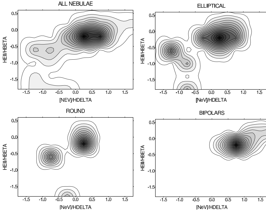
Fig. 4. As for Fig. 1, but for the He II/H \beta -[Ne V]/H \delta plane. Note the presence of at least two subsets of circular and elliptical PNe, having higher and lower values of [Ne V]/H \delta .
