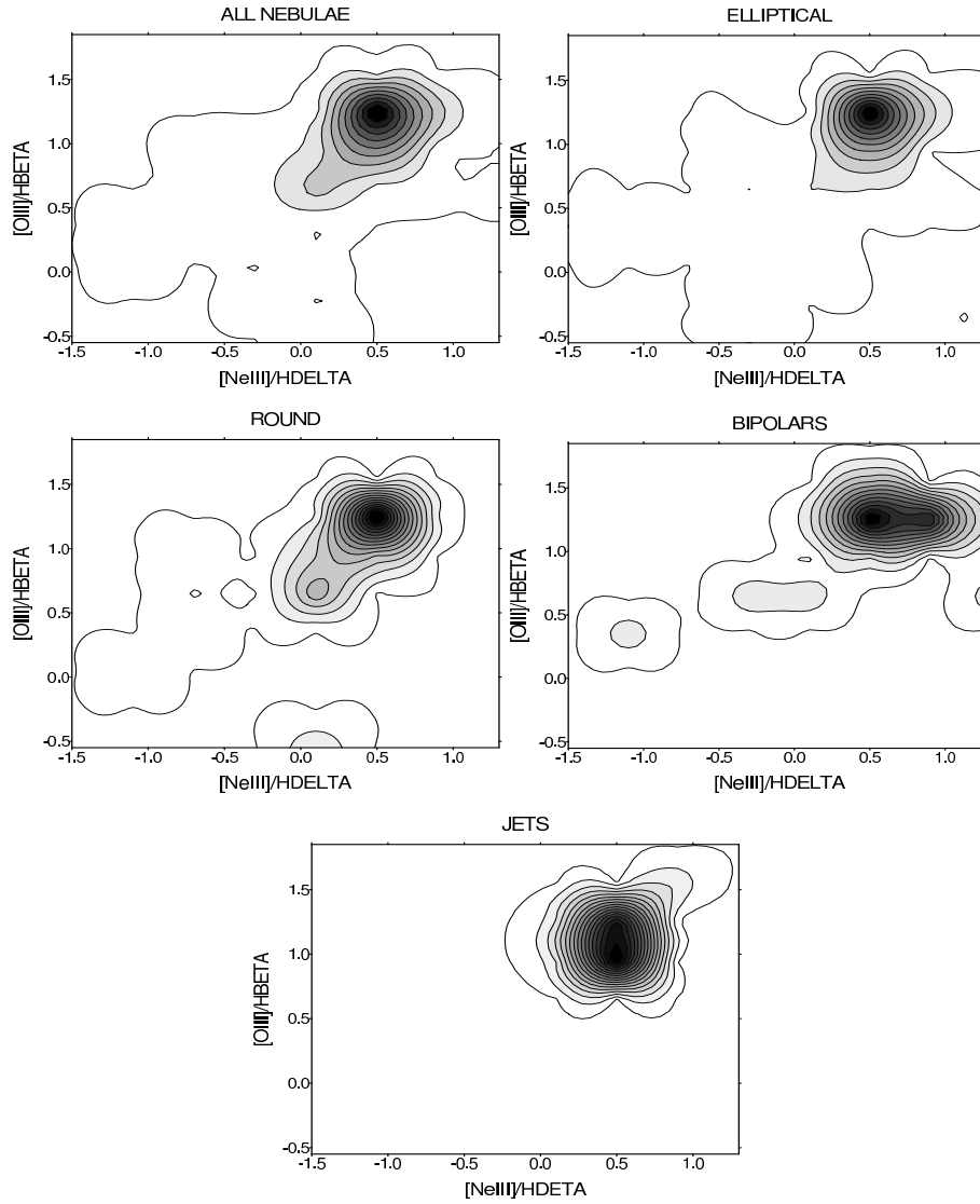
Fig. 6. As in Fig. 1, but for the [O\ III]/H\beta – [Ne\ III]/H\delta plane. Note the very restricted ranges of line ratio characterizing most PNe.
