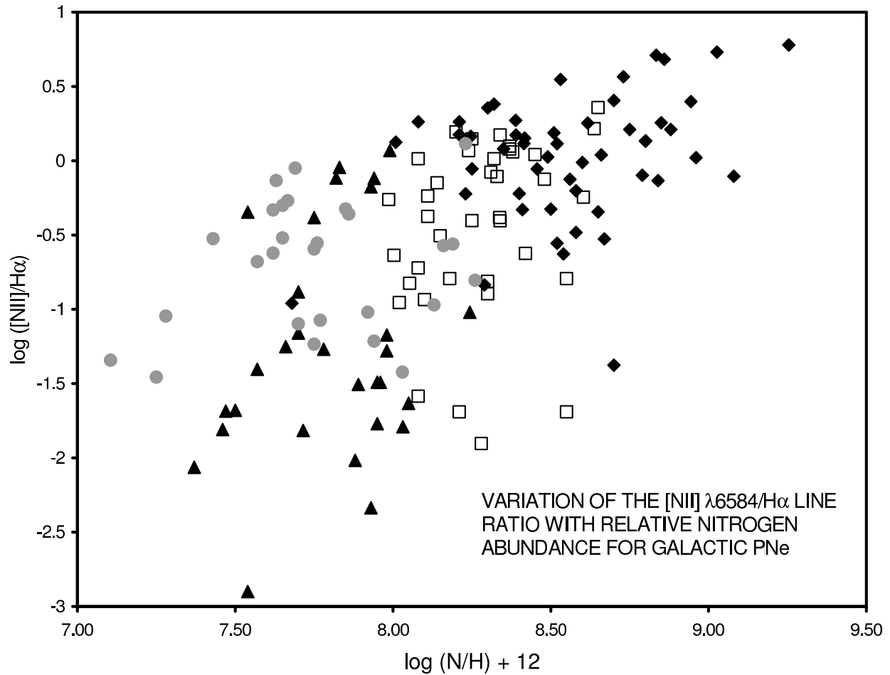
Fig. 10. Variation of relative nitrogen abundance with [\text{N II}]/\text{H}\alpha for Galactic planetary nebulae. We have identified Type I (filled lozenges), Type IIa (open squares), Type IIb (filled triangles), and Type III (grey filled circles) PNe.
