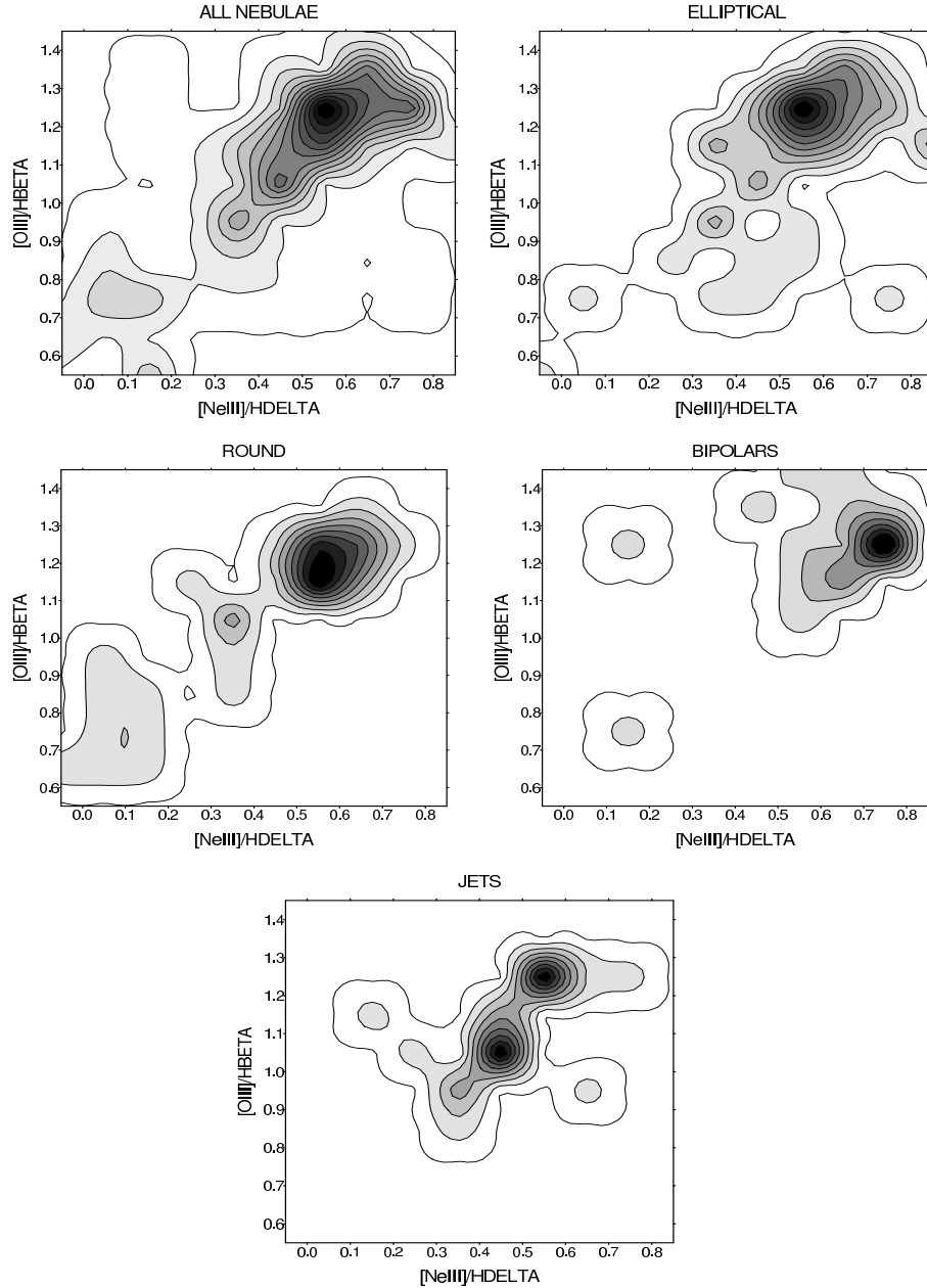
Fig. 7. As in Fig. 6, but at much higher resolution (note the change in axial ranges). We note similar tendencies for the jets and bipolar sources to those noted in previous figures.
