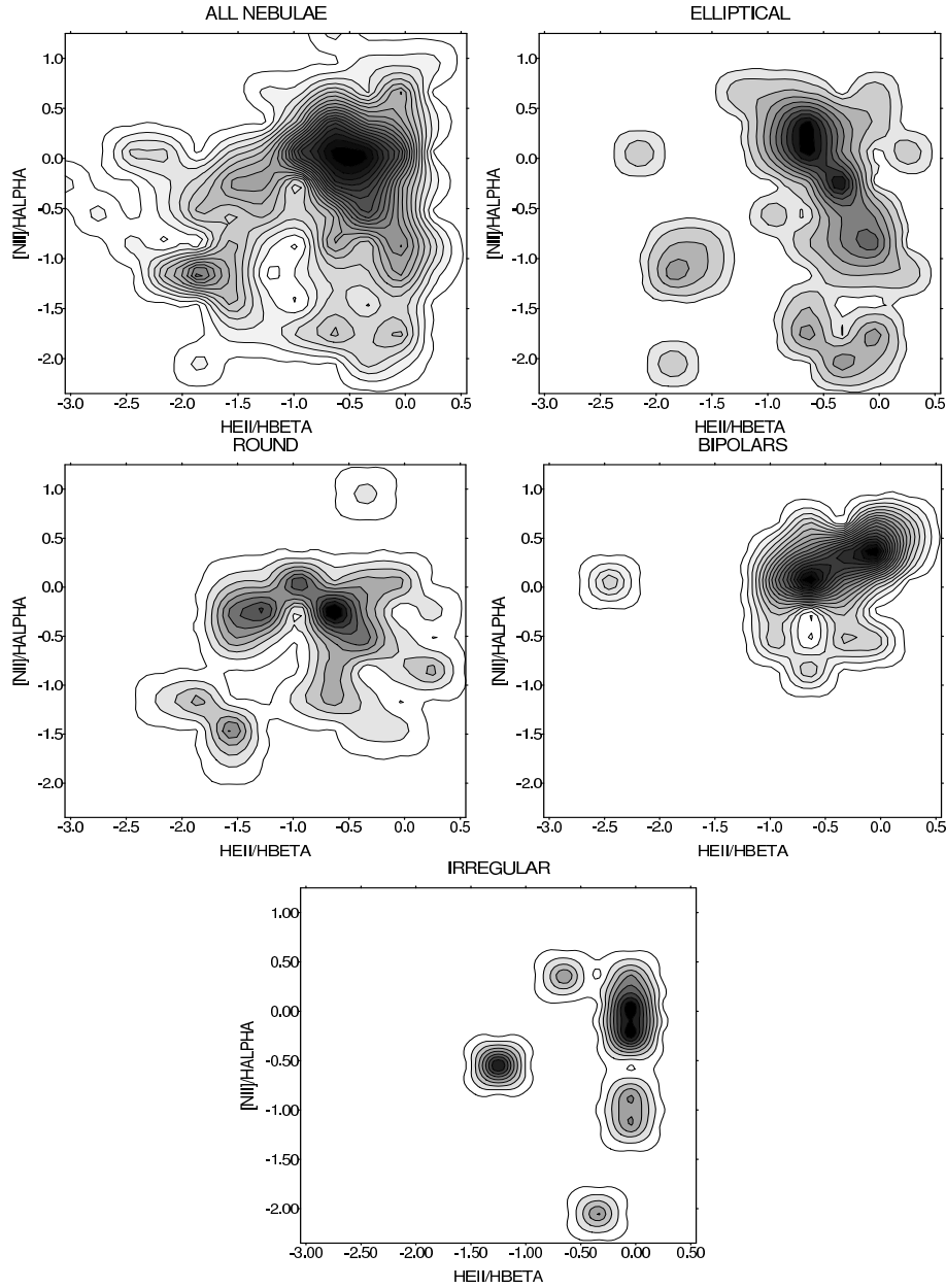
Fig. 5. As in Fig. 1, but for the [\text{N II}]/\text{H}\alpha – \text{He II}/\text{H}\beta plane. It is apparent that the irregular sources tend to congregate towards the right-hand side of the map, where values of \text{He II}/\text{H}\beta are appreciable.
