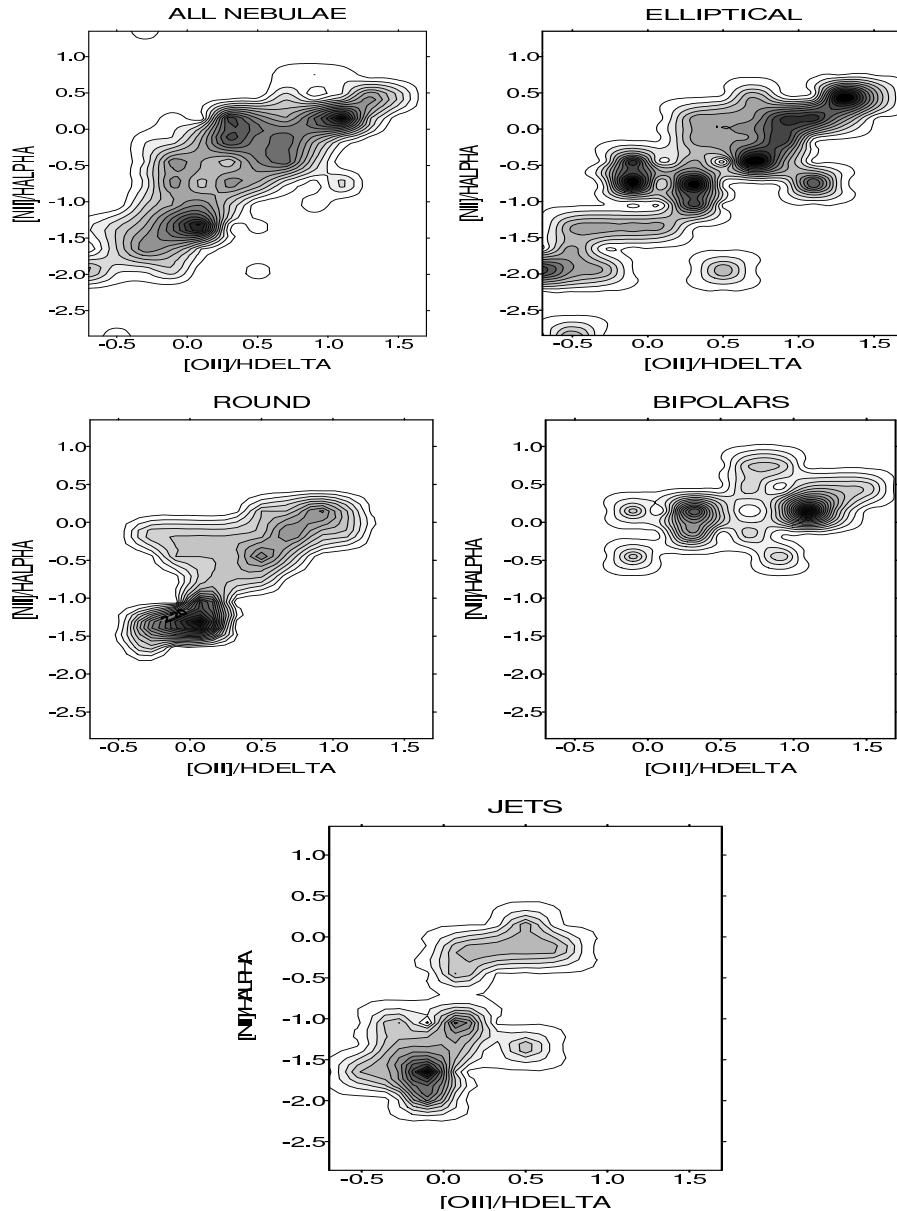
Fig. 1. Distribution of differing morphological classes of PNe within the [\text{N II}]/\text{H}\alpha – [\text{O II}]/\text{H}\delta plane. Line ratios are given in logarithmic units, whilst contour levels are set at linear intervals, and refer to the density of sources within this plane. Note the tendency for bipolar nebulae to be located towards high values of line ratio, and of circular sources to be concentrated towards lower line ratios. Elliptical sources appear to occupy the full gamut of ratios, from the very low to the very high.
