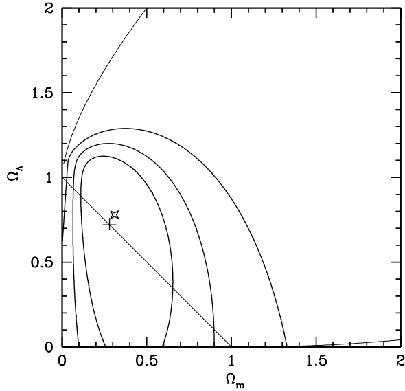
Fig. 1. Contours at 68.3%, 95.5%, and 99.7% CL's obtained by projecting on the (\Omega_m, \Omega_\Lambda) plane the L_{\text{iso}}-E_{\text{pk}}-T_{0.45} relation \chi_r^2 derived from the fit of the GRB data at each value of the (\Omega_m, \Omega_\Lambda) pair. The star shows where the \chi_r^2 reaches its minimum, while the cross indicates the concordance cosmology. This plot shows that the relation L_{\text{iso}}-E_{\text{pk}}-T_{0.45} is sensitive to cosmology, so that it may be used to discriminate cosmological parameters if an optimal method to circumvent the circularity problem is used. The diagonal line corresponds to the flat geometry cosmology, the upper curve is the loitering limit between Big Bang and No Big Bang models, and the lower curve indicates the division between accelerating and non-accelerating universes.
