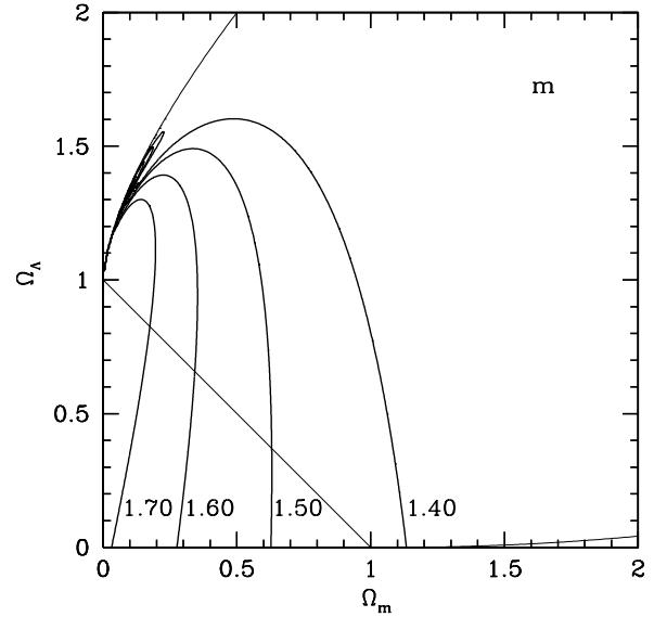
Fig. 2. Contours of constant m in the (\Omega_m, \Omega_\Lambda) plane. m is the power of E_{\text{pk}} in the L_{\text{iso}}-E_{\text{pk}}-T_{0.45} relation: L_{\text{iso}} \propto E_{\text{pk}}^m T_{0.45}^{-n} . The other curves in the plot are as in Figure 1.
