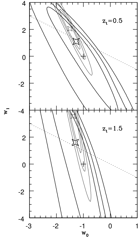
Fig. 10. Constraints on the (w_0, w_1) plane for a flat cosmology with dynamic DE and \Omega_m = 0.28 from the GRB Hubble diagram using the Bayesian formalism to solve optimally the circularity problem (thick-line ellipses) and from the “gold set” SNIa Hubble diagram (thin-line ellipses). Upper and lower panels are for z_t = 0.5 and z_t = 1.5 , respectively. The ellipses are contours at 68.3%, 95.5%, and 99.7% CL’s. The diagonal dot-dashed line is the upper limit in the (w_0, w_1) -plane allowed by CMB constraints.
