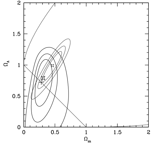
Fig. 8. Constraints on the (\Omega_m, \Omega_\Lambda) plane for a \Lambda cosmology from the GRB Hubble diagram using our Bayesian method to circumvent the circularity problem (thick-line ellipses) and from the “gold set” SNIa Hubble diagram (thin-line ellipses). The ellipses are contours at 68.3%, 95.5%, and 99.7% CL’s. The other curves in the plot are as in Figure 1.
