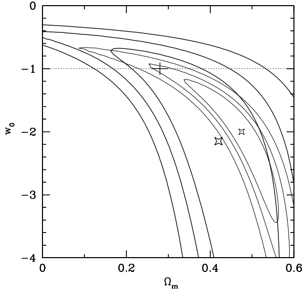
Fig. 9. Constraints on the (\Omega_m, w) plane for a flat cosmology with static DE from the GRB Hubble diagram using the Bayesian formalism to solve optimally the circularity problem (thick-line ellipses) and from the “gold set” SNIa Hubble diagram (thin-line ellipses). The bent ellipses are contours at 68.3%, 95.5%, and 99.7% CL’s.
