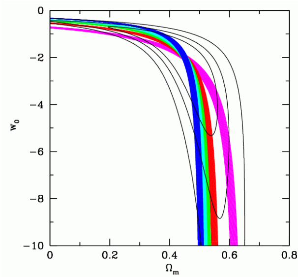
Fig. 6. Same as Figure 5 but in the (\Omega_m, w) plane for a flat cosmology with static DE. The fiducial point is (\Omega_m, w) = (0.45, -2.00) . Taking the vertical regions of the stripes, the redshifts are 0.5, 1.0, 1.5, 2.0, and 3.0 from right to left, respectively [in the electronic version of this paper z = 0.5 (magenta), 1.0 (red), 1.5 (green), 2.0 (cyan), and 3.0 (blue)]. For low values of \Omega_m , w is almost independent from \Omega_m , while the opposite happens for high values of \Omega_m . The dependence of the \Omega_m - w degeneracy on z is weak. As in Figure 5, the bent ellipses are the contours of CL for the corresponding GRB Hubble diagram, using a L_{\text{iso}}-E_{\text{pk}}-T_{0.45} relation supposed to be known, and therefore fixed and cosmology-independent.
