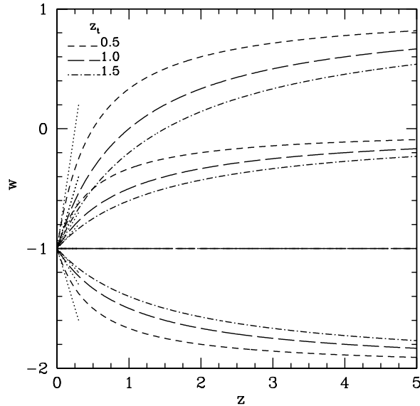
Fig. 4. Dependence of the equation of state parameter w on z as described by Eq. (2). For the plot, w_0 = -1 is assumed. Values of w_1 = 2, 1, 0 and -1 (from top to bottom respectively) and of z_t = 0.5, 1.0, 1.5 (see labels inside the panel) for each w_1 are used. The dotted lines are the tangent lines of each curve at z = 0 and represent the linear approximation.
