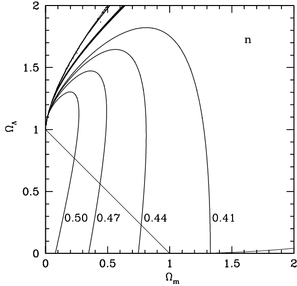
Fig. 3. Contours of constant n in the (\Omega_m, \Omega_\Lambda) plane. n is the power of T_{0.45} in the L_{\text{iso}}-E_{\text{pk}}-T_{0.45} relation: L_{\text{iso}} \propto E_{\text{pk}}^m T_{0.45}^{-n} . The other curves in the plot are as in Figure 1.
