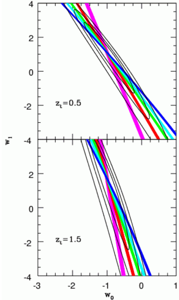
Fig. 7. Same as Figure 5 but in the (w_0, w_1) plane for a flat geometry cosmology with dynamic DE and \Omega_m = 0.28 . The evolving w(z) is parametrized according to Eq. (2) with z_t = 0.5 (upper panel) and z_t = 1.5 (lower panel). The fiducial points are (w_0, w_1) = (-1.00, 1.08) and (w_0, w_1) = (-1.01, 0.61) , respectively. Taking the lower part of the stripes, the redshifts are 0.5, 1.0, 1.5, 2.0 and 3.0 from left to right, respectively [in the electronic version of this paper z = 0.5 (magenta), 1.0 (red), 1.5 (green), 2.0 (cyan), and 3.0 (blue)]. As in Figure 5, the ellipses are the contours of CL from the corresponding GRB Hubble diagram, using a L_{\text{iso}}-E_{\text{pk}}-T_{0.45} relation supposed to be known, and therefore fixed and cosmology-independent.
