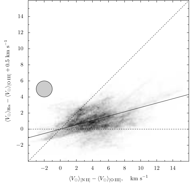
Fig. 22. Joint distribution of differences in mean velocities: \langle V \rangle_{\text{H}\alpha} - \langle V \rangle_{\text{O III}} versus \langle V \rangle_{\text{N II}} - \langle V \rangle_{\text{O III}} . The values of \langle V \rangle_{\text{H}\alpha} - \langle V \rangle_{\text{O III}} have been shifted by 0.5 \text{ km s}^{-1} so as to make the distribution symmetric about a line through the origin (see discussion in text). The dashed lines show the boundaries of the two triangular regions (upper right and lower left) that give physically possible values of f in the two-zone model. The solid line shows the relationship \langle V \rangle_{\text{H}\alpha} - \langle V \rangle_{\text{O III}} = (1 - \langle f \rangle)(\langle V \rangle_{\text{N II}} - \langle V \rangle_{\text{O III}}) , where \langle f \rangle is determined from the R_{\text{N II}} method. The solid gray circle indicates the effect of \pm 1 \text{ km s}^{-1} uncertainties in the velocities.
