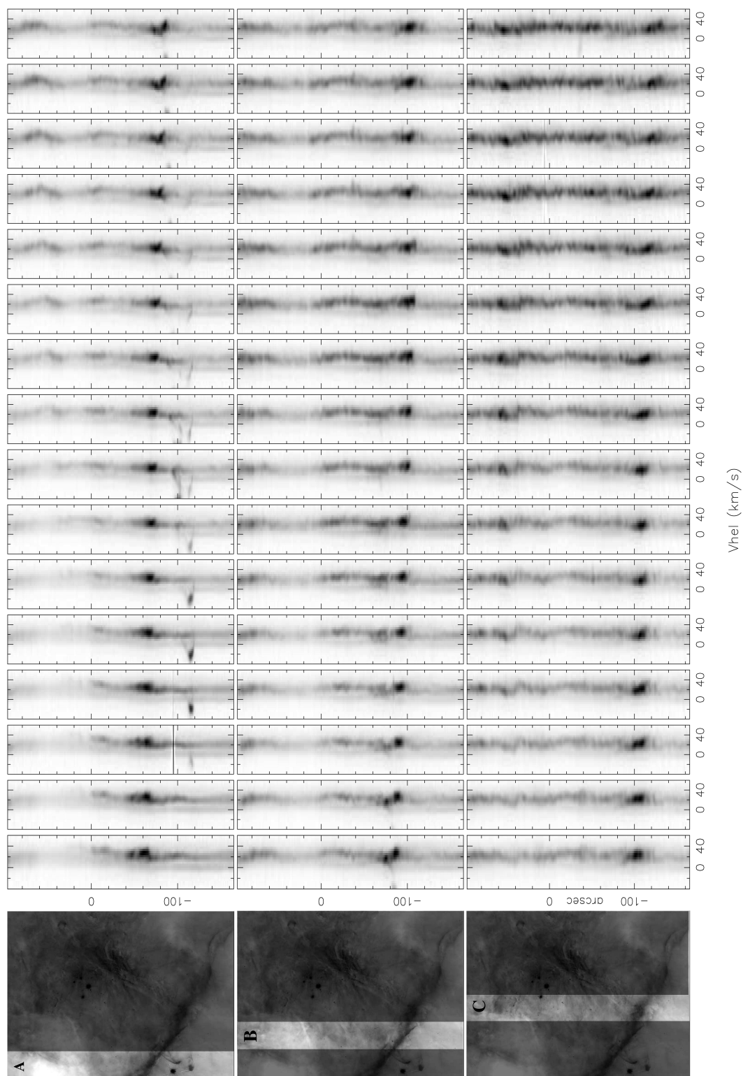
Fig. 8: As Figure 1 but for [\text{N II}] 6584 Å.
