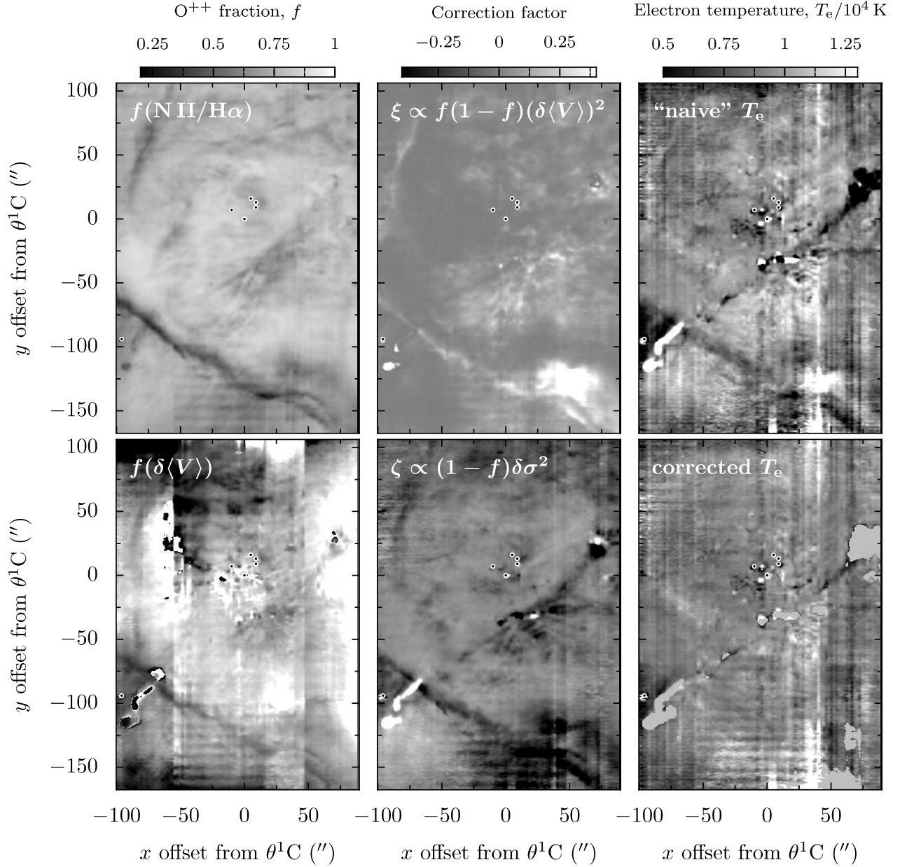
Fig. 21. Steps in the construction of the temperature map. Left column: Two independent estimates of the fraction, f , of the H\alpha emission that comes from the O^{++} zone: from the [N\ II]/H\alpha surface brightness ratio (upper panel), and from the differences in mean velocities of [N\ II] , H\alpha , [O\ III] (lower panel). Center column: Correction factors to the “naive” temperature map due to differences in the kinematics between the N^+ and O^{++} zones: mean velocity differences, \xi (upper panel) and velocity dispersion differences, \zeta (lower panel). Right column: “naive” temperature estimate (upper panel) from the difference in velocity dispersion of [O\ III] and H\alpha and final corrected temperature estimate (lower panel). The horizontal bands and vertical streaks seen in some panels are instrumental artifacts.
