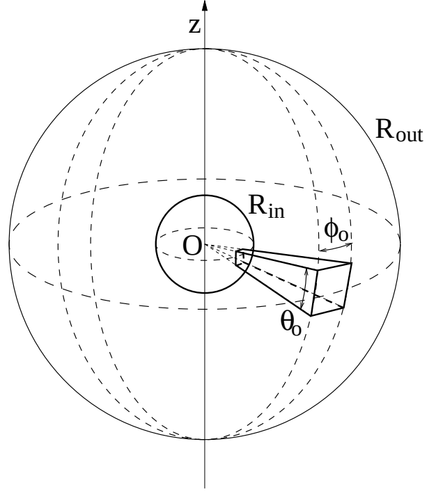
Fig. 2. Schematic geometry of the accretion column onto the neutron star surface.
