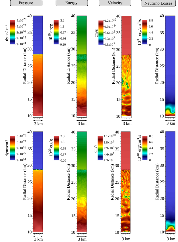
Fig. 4. Color maps of pressure, total specific energy, magnitude of velocity and neutrino emissivity, for cases HYDRO (top) and MHD_0 (bottom) at t = 10 ms. The accretion rate is \dot{M} = 100 \dot{M}_0 .
