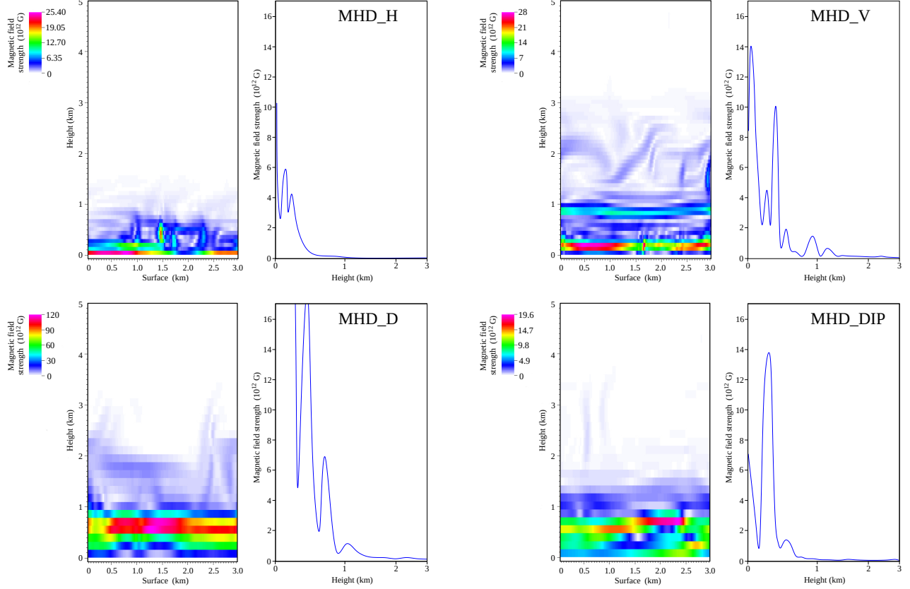
Fig. 10. Maps (left half-panel) and horizontally-averaged vertical profiles (right half-panel) of magnetic field strength for a magnetic field that is initially horizontal, case MHD_H (top left), vertical, case MHD_V (top right), diagonal, case MHD_D (bottom left), and dipolar, case MHD_DIP (bottom right), after the system has relaxed for \dot{M} = 1000\dot{M}_0 . Note the submergence of the magnetic field close to the neutron star surface.
