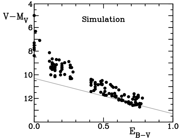
Fig. 4. A simulated variable-extinction diagram for a star field where the reddening increases with distance according to dust clouds producing E_{B-V} = 0.20, 0.50, and 0.70 located at distances of 0.5 kpc, 0.9 kpc, and 1.1 kpc, respectively, with associated uncertainties in E_{B-V} of \pm 0.05 and in M_V of \pm 0.5 . The gray line denotes a standard reddening law of R = A_V/E_{B-V} = 3.0 for stars at a distance of 1.1 kpc.
