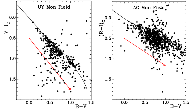
Fig. 2. Two-color diagrams, V-I_C versus B-V for the field of UY Mon (left), and (R-I)_C versus B-V for the field of AC Mon (right), showing the intrinsic color relations adopted (solid curves). Reddening lines specific for the fields are shown separately in red for E_{B-V} = 1.0 , with arrows denoting the direction of increasing reddening. The color figure can be viewed online.
