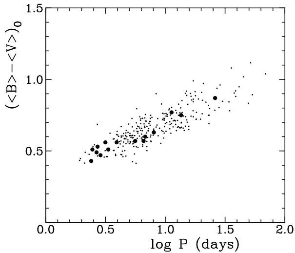
Fig. 6. Derived intrinsic \langle B \rangle - \langle V \rangle_0 colors for sample Cepheids (large symbols) relative to other Cepheids with derived reddenings (small symbols, Turner 2001), as a function of pulsation period.
