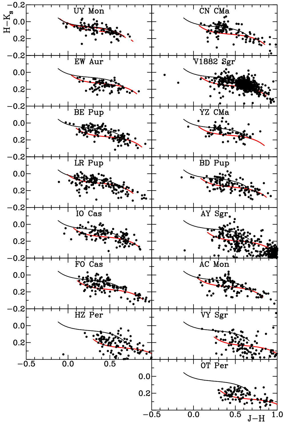
Fig. 5. 2MASS color-color diagrams, H-K_s versus J-H , for stars within 5' of each Cepheid, from observations by Cutri et al. (2003). The intrinsic relation for main sequence stars is plotted as a black line, while red lines depict the adopted reddening for stars associated with the Cepheids, from Column 7 of Table 2. The dashed red line for UY Mon represents the alternate solution for that field. The color figure can be viewed online.
