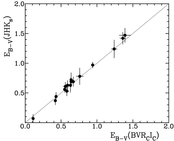
Fig. 8. Comparison of derived 2MASS reddening, with their uncertainties, for the Cepheids in our sample with the color-corrected broad band BV(RI)_C reddening. The gray line represents expectations for an exact match.
