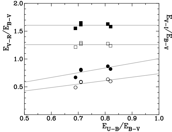
Fig. 1. Derived Johnson system (filled symbols) and Kron-Cousins system (open symbols) reddening ratios E_{V-R}/E_{B-V} (circles, lower) and E_{V-I}/E_{B-V} (squares, upper) for fields studied by Johnson (1968). Gray lines denote the implied dependences on reddening slope E_{U-B}/E_{B-V} .
