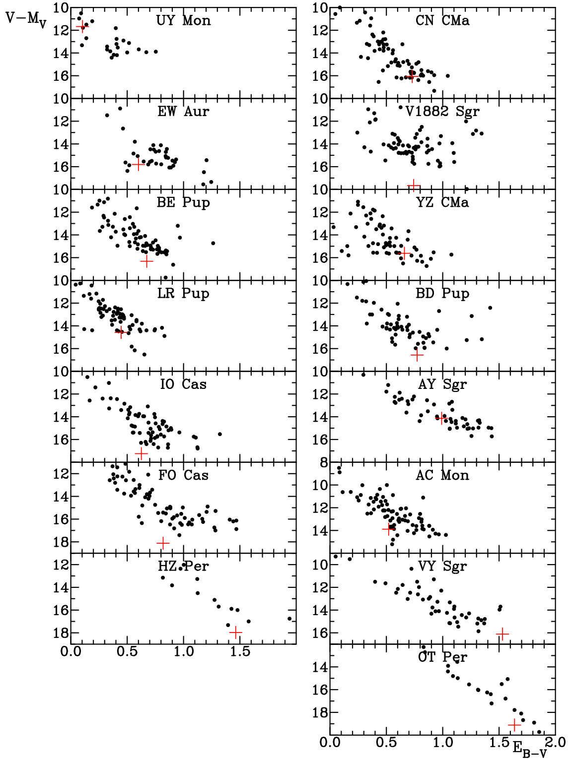
Fig. 3. Variable-extinction diagrams for the fields examined in this study, identified by the Cepheid of interest. Filled symbols denote AF stars near each Cepheid, and red plus signs are “predictions” for the Cepheid parameters. The color figure can be viewed online.
