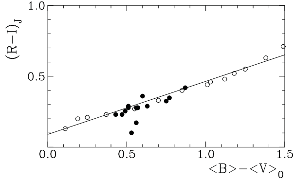
Fig. 7. Derived Johnson system (R-I)_J colors for sample Cepheids (filled circles) relative to intrinsic (\langle B \rangle - \langle V \rangle)_0 colors, with derived colors for AFGK supergiants from Johnson (1966) plotted for reference purposes as open circles. The line is a fitted relation for the supergiants. The anomalous Cepheids are V1882 Sgr and YZ CMa.
