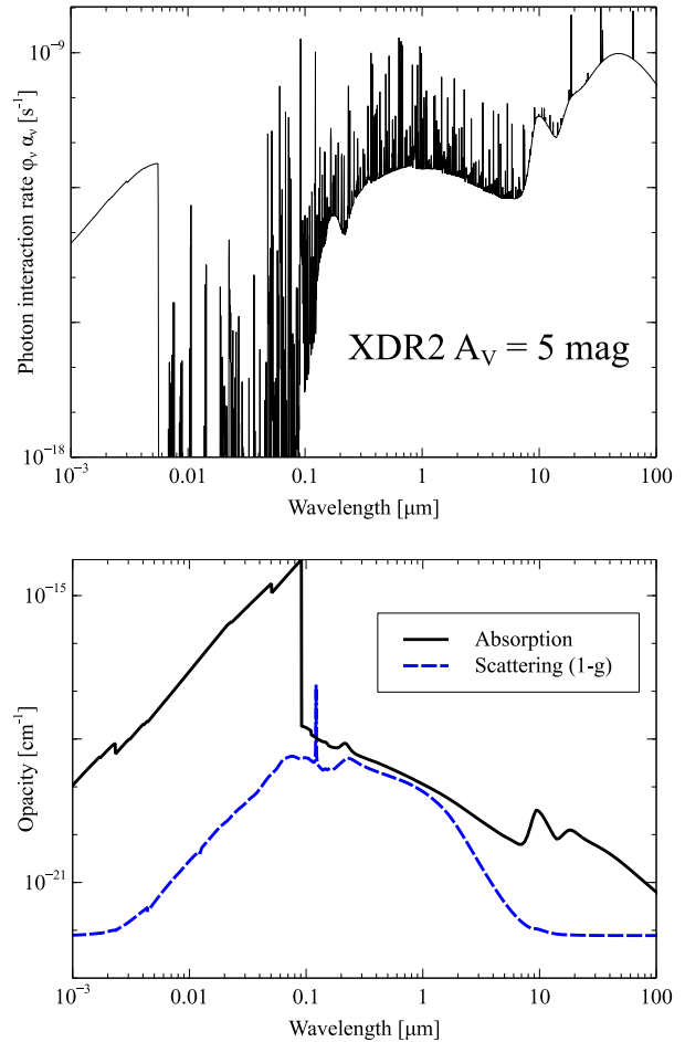
Fig. 7. Components of the radiation field at a depth corresponding to A_V = 5 mag in the XDR2 simulation. The lower panel shows the absorption and scattering opacities while the upper panel shows the photon interaction rate.
