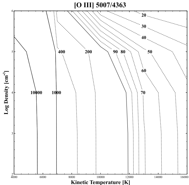
Fig. 2. The [O III] line \lambda\lambda 5007/4363 intensity ratio as a function of density and temperature.
