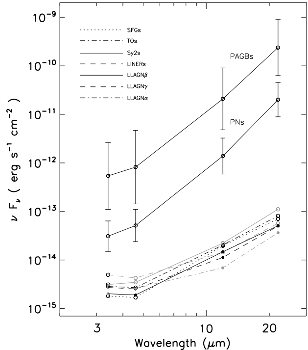
Fig. 12. The mean MIR fluxes at the four different wavelengths used by WISE. How one transforms the WISE magnitudes into fluxes is explained in Wright et al. (2010). The error bars for the stars are the errors on the means (Bevington & Robinson 2003). For clarity sake, the errors on the mean for the galaxies are shown only in Figure 12.
