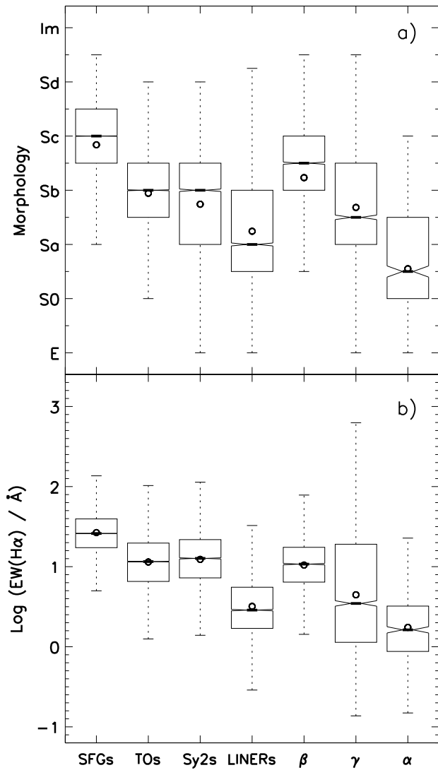
Fig. 11. Box-whisker plots comparing a) the morphologies of the NELGs in our sample, and b) their H\alpha EWs. The explanations for the box-whisker plots and identification of the samples are as in Figure 9.
