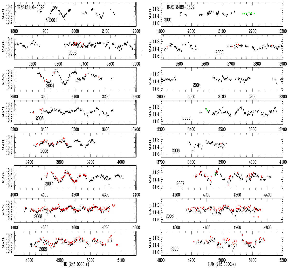
Fig. 3. Light variations in the stars IRAS13110–6629 and IRAS18489–0629 as seen from the V-band data from the All Sky Automated Survey. Each independent data set is depicted with a different color. Year numbers are placed at the beginning of the calendar year for a reference. See § 2.1. for more details. The color figure can be viewed online.
