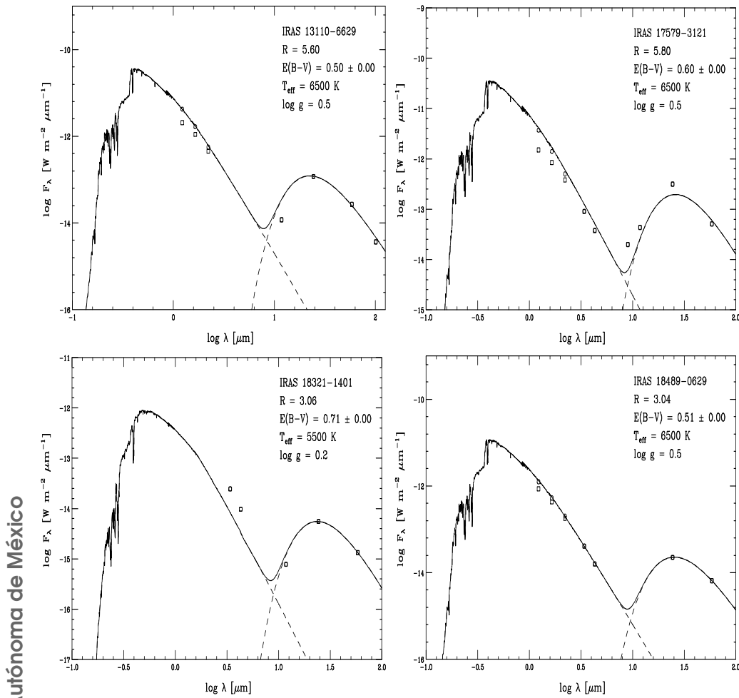
Fig. 5. The ED for the program stars is generated using the existing photometric data and IR colors as described in the text.
