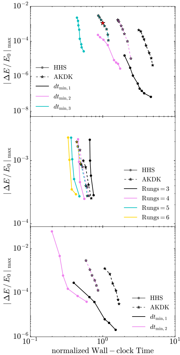
Fig. 6. Energy conservation as a function of wall-clock time (normalized with respect to the red star case in upper panel) for the fiducial isolated halo (upper and middle panels) and for a cuspy halo including four live cuspy satellites (bottom panel), for the HHS (solid circles) and AKDK (stars) integrators. In the upper panel, we used a Plummer softening \epsilon = 0.007 , and we varied the minimum time step ( dt_{\min,1} = 5.4 \times 10^{-3} , dt_{\min,2} = 1.1 \times 10^{-2} and dt_{\min,3} = 2.2 \times 10^{-2} ) but fixing the number of rungs (6 and 5 for HHS and AKDK, respectively). In the middle panel, we used \epsilon = 0.01 , and we varied the number of rungs, but fixed the minimum time step ( dt_{\min} = 4.3 \times 10^{-2} ). For the bottom panel, we used \epsilon = 0.004 , and we varied the minimum time step ( dt_{\min,1} = 6.4 \times 10^{-3} and dt_{\min,2} = 1.3 \times 10^{-2} ) but fixing the number of rungs (6 and 3 for HHS and AKDK, respectively). The color figure can be viewed online
