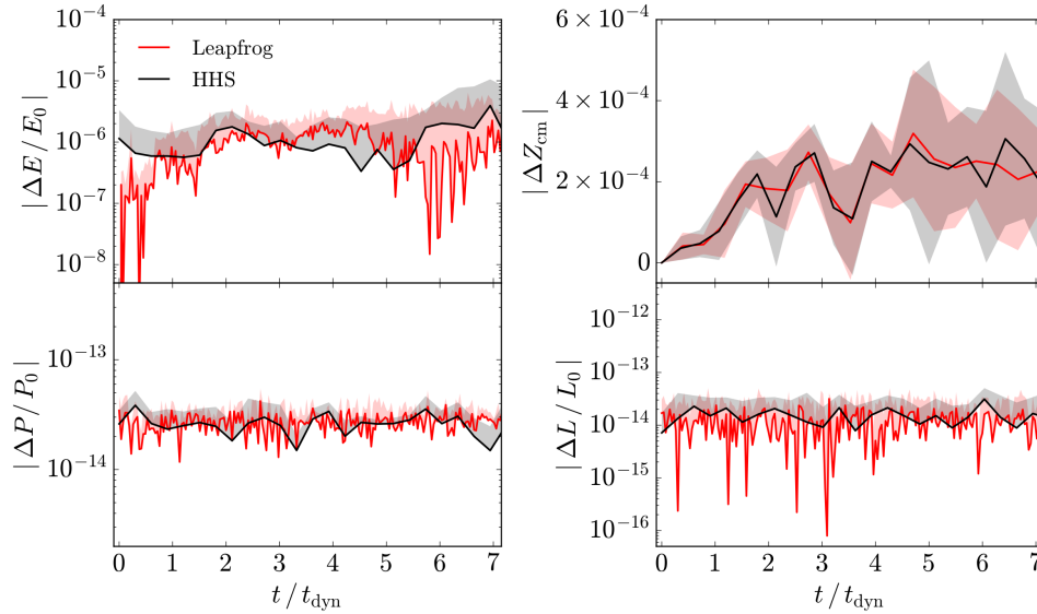
Fig. 10. Error in conserved quantities for a NFW halo with N = 10^5 particles plus a satellite simulated up to 7 dynamical times. Shown is the energy error (upper left panel), the change in center of mass position (upper right panel), the error in linear (lower left panel) and angular momentum (lower right panel) for the Leapfrog (red) and HHS (black) integrators. Shaded portions represent one sigma standard deviation propagated from different realizations ran under different random seeds. The color figure can be viewed online.
