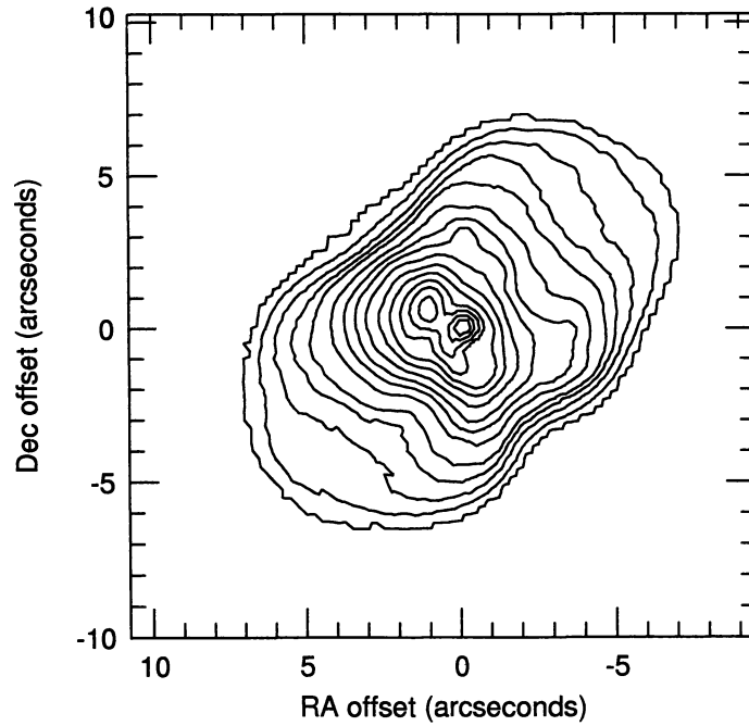
Fig. 1. 12.5 \mu\text{m} surface brightness in \eta Carinae. Contours are at 2,3,5,7,8,12,15,20,25,33,42,50,67,83,95 per cent of the peak. The pixel scale is 0.25'' and the spatial resolution is \sim 0.75''
